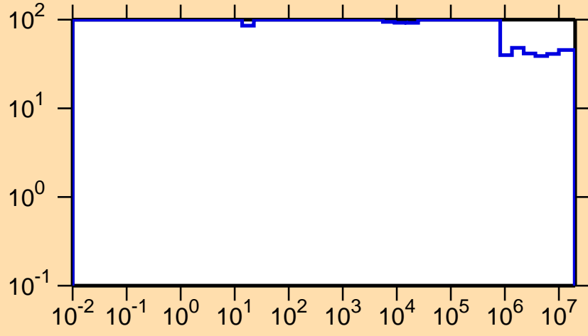
\Delta\sigma/\sigma vs. E for ^{218}\text{At}(n,\text{nonel.})
