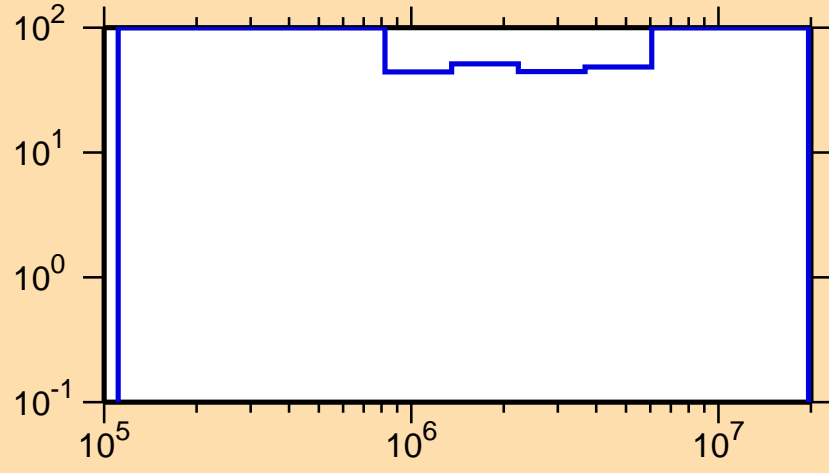
\Delta\sigma/\sigma vs. E for ^{218}\text{At}(n,\text{inel.})
