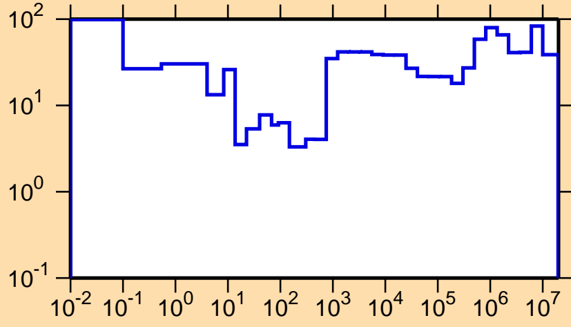
\Delta\sigma/\sigma vs. E for ^{218}\text{At}(n,el.)
