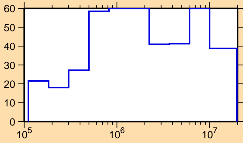
\Delta\sigma/\sigma vs. E for ^{218}\text{At}(n,\text{el.})
