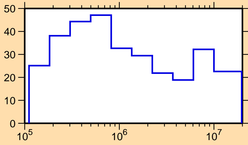
\Delta\sigma/\sigma vs. E for ^{218}\text{At}(n,\text{tot.})
