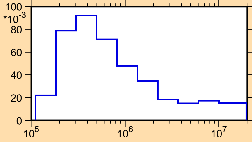
\sigma vs. E for ^{218}\text{At}(n,n_1)
