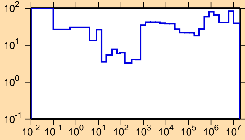
\Delta\sigma/\sigma vs. E for ^{218}\text{At}(n,\text{el.})
