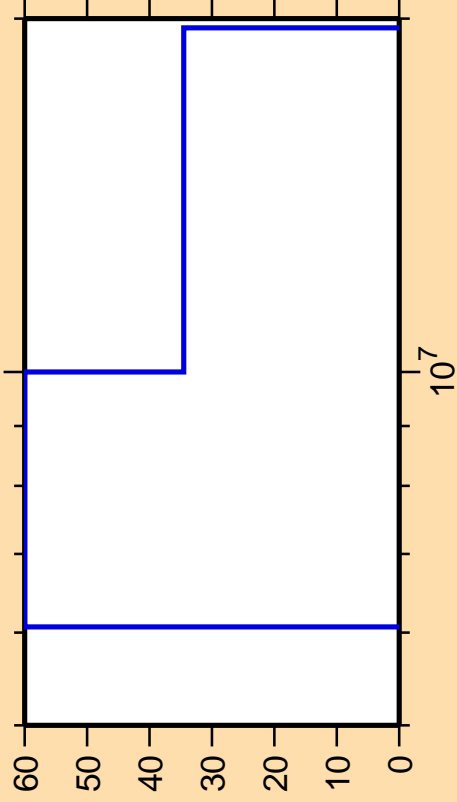
\Delta\sigma/\sigma vs. E for ^{218}\text{At}(n,np)
