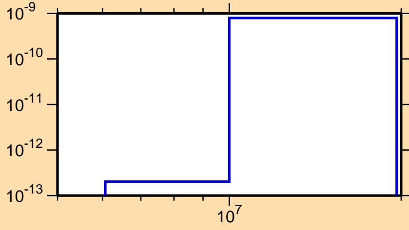
\sigma vs. E for ^{218}\text{At}(n,p\alpha)
