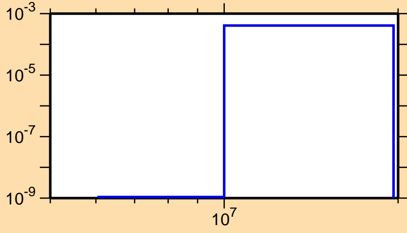
\sigma vs. E for ^{218}\text{At}(n,np)
