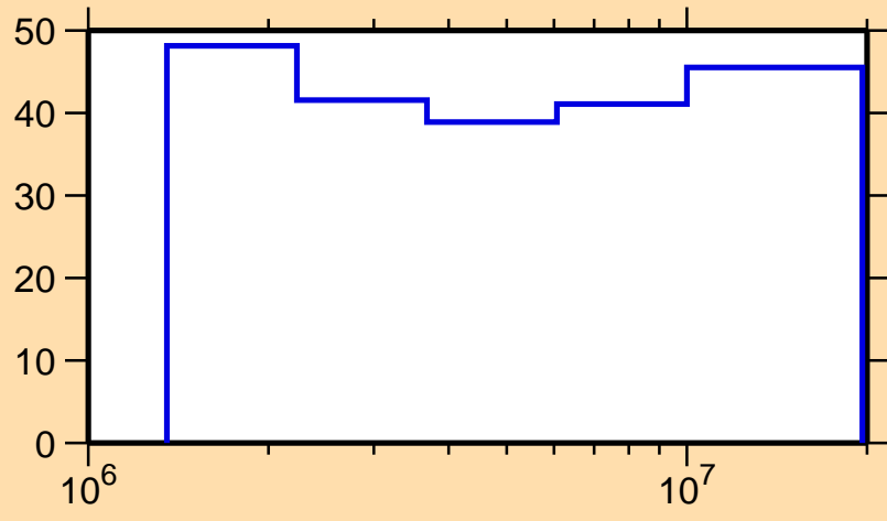
\Delta\sigma/\sigma vs. E for ^{218}\text{At}(n,\text{nonel.})
