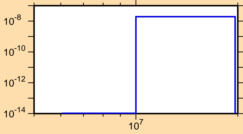
\sigma vs. E for ^{218}\text{At}(\text{mt } 45)
