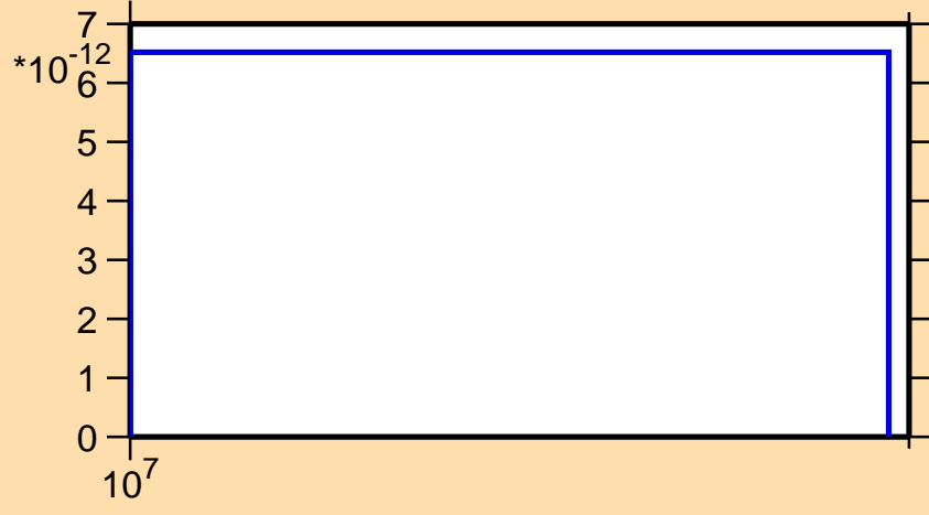
\sigma vs. E for ^{218}\text{At}(n,\text{He3})
