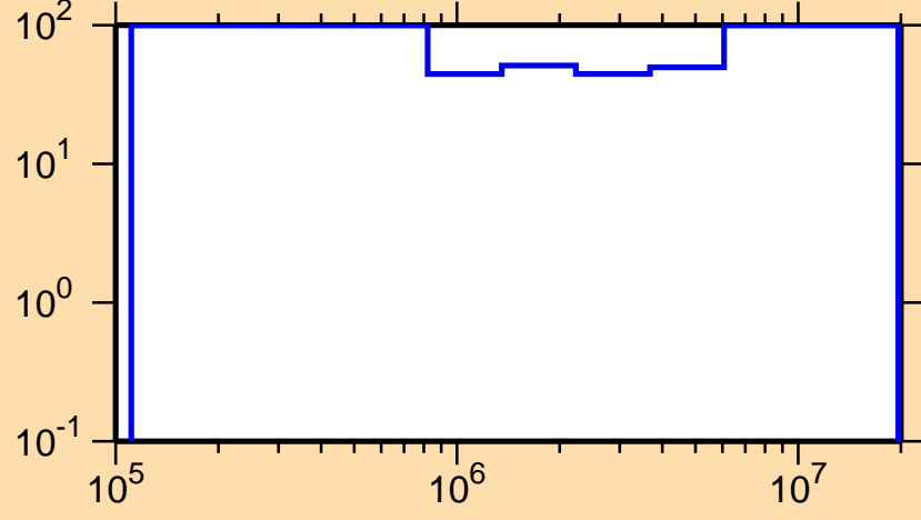
\Delta\sigma/\sigma vs. E for ^{218}\text{At}(n,n\text{cont.})
