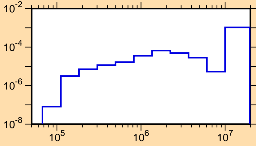
\sigma vs. E for ^{218}\text{At}(n,n\alpha)
