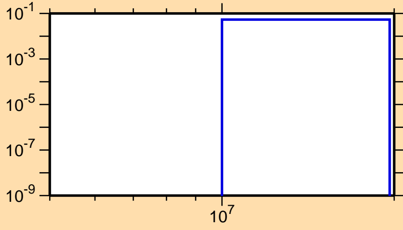
\sigma vs. E for ^{218}\text{At}(n,3n\alpha)
