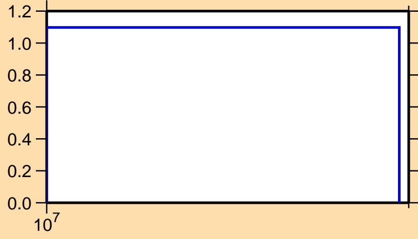
\sigma vs. E for ^{218}\text{At}(n,3n)
