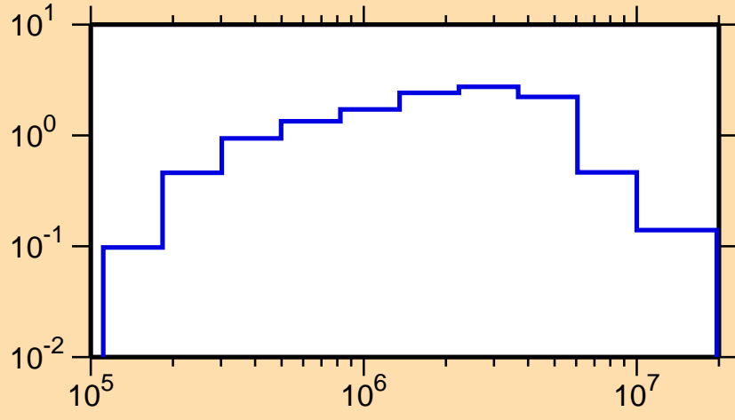
\sigma vs. E for ^{218}\text{At}(n,\text{inel.})
