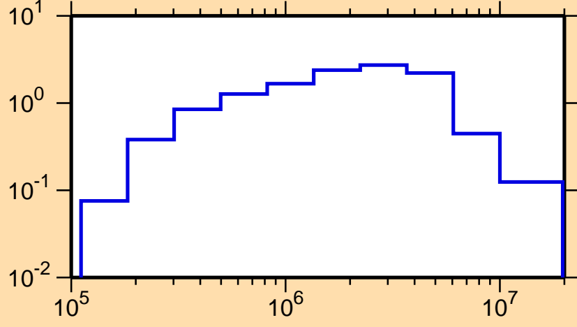
\sigma vs. E for ^{218}\text{At}(n,n\text{cont.})
