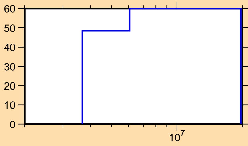
\Delta\sigma/\sigma vs. E for ^{218}\text{At}(n,\text{inel.})
