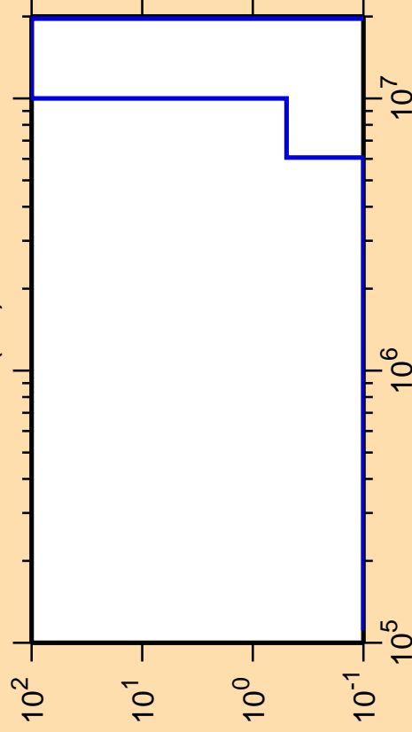
\Delta\sigma/\sigma vs. E for ^{218}\text{At}(n,f)
