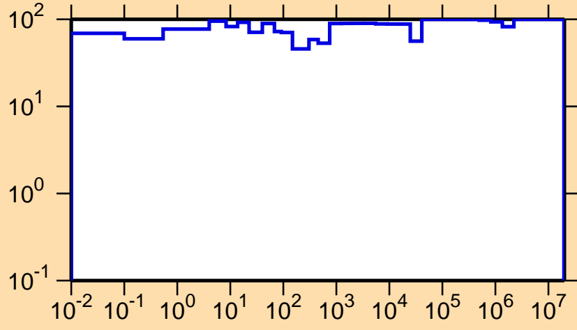
\Delta\sigma/\sigma vs. E for ^{218}\text{At}(n,\gamma)
