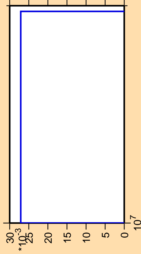
\Delta\sigma/\sigma vs. E for ^{218}\text{At}(\text{mt } 34)
