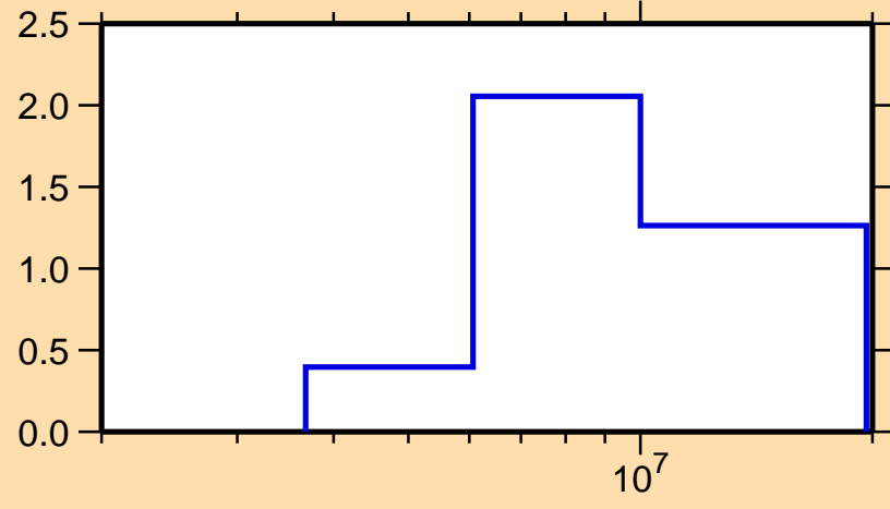
\sigma vs. E for ^{218}\text{At}(n,2n)
