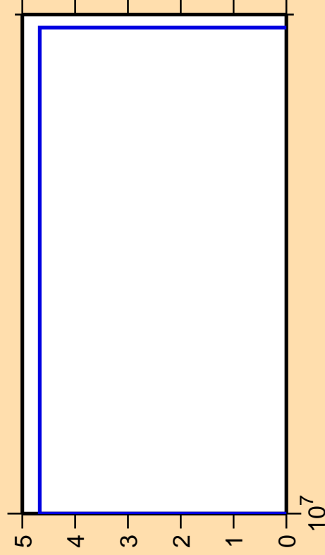
\Delta\sigma/\sigma vs. E for ^{218}\text{At}(\text{mt } 42)
