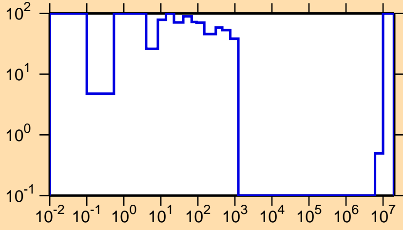
\Delta\sigma/\sigma vs. E for ^{218}\text{At}(n,f)
