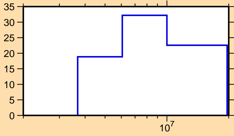
\Delta\sigma/\sigma vs. E for ^{218}\text{At}(n,\text{tot.})
