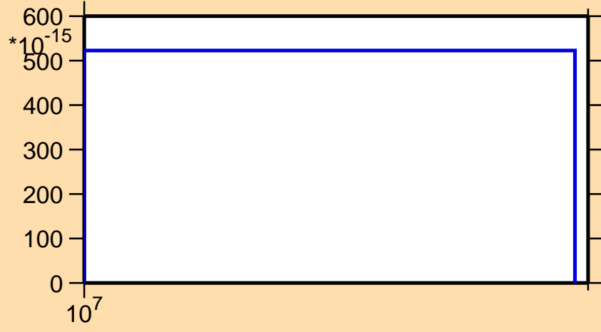
\sigma vs. E for ^{218}\text{At}(\text{mt } 42)
