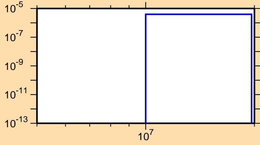
\sigma vs. E for ^{218}\text{At}(n,\text{nd})
