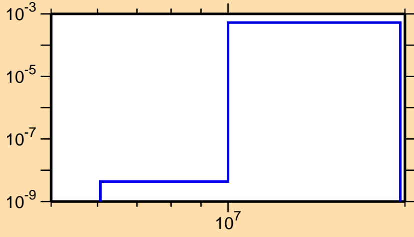
\sigma vs. E for ^{218}\text{At}(n,d)
