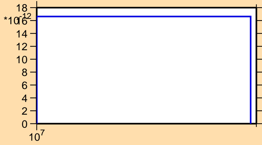
\sigma vs. E for ^{218}\text{At}(\text{mt } 11)
