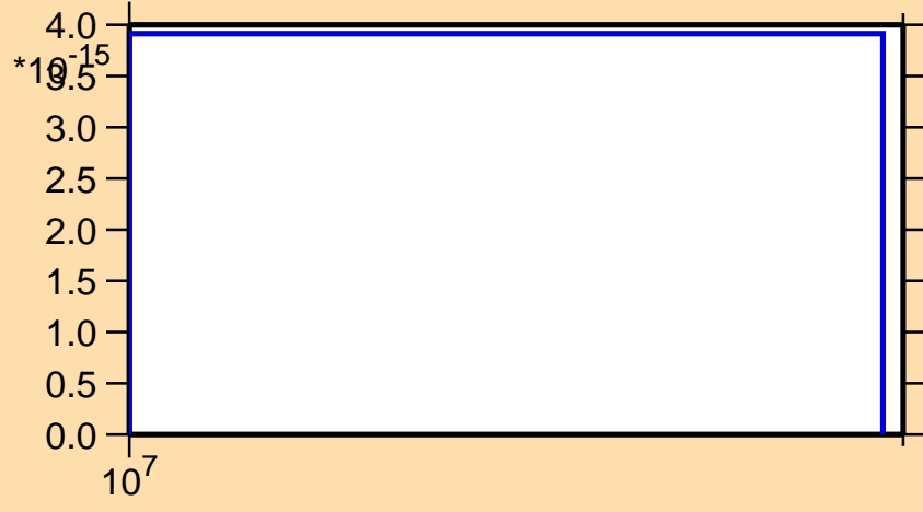
\sigma vs. E for ^{218}\text{At}(\text{mt } 34)
