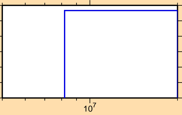
\sigma vs. E for ^{218}\text{At}(n,\text{He3})
