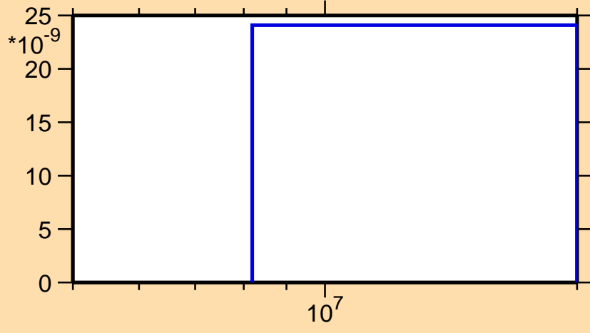
\sigma vs. E for ^{218}\text{At}(\text{mt117})
