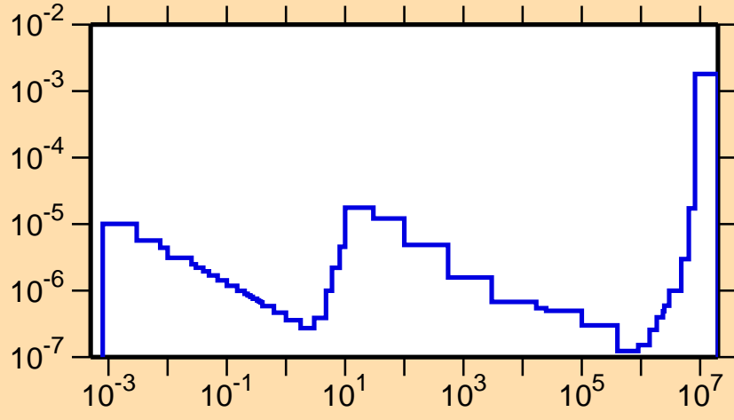
\sigma vs. E for ^{218}\text{At}(n,\alpha)
