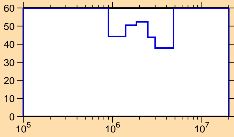
\Delta\sigma/\sigma vs. E for ^{218}\text{At}(n,n\text{cont.})
