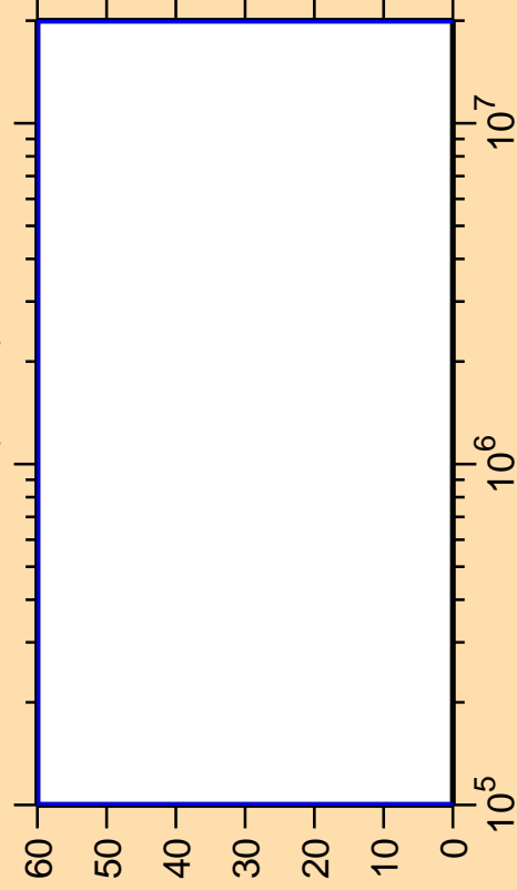
\Delta\sigma/\sigma vs. E for ^{218}\text{At}(n,n\alpha)
