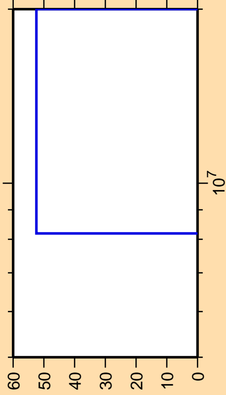
\Delta\sigma/\sigma vs. E for ^{218}\text{At}(n,nd)
