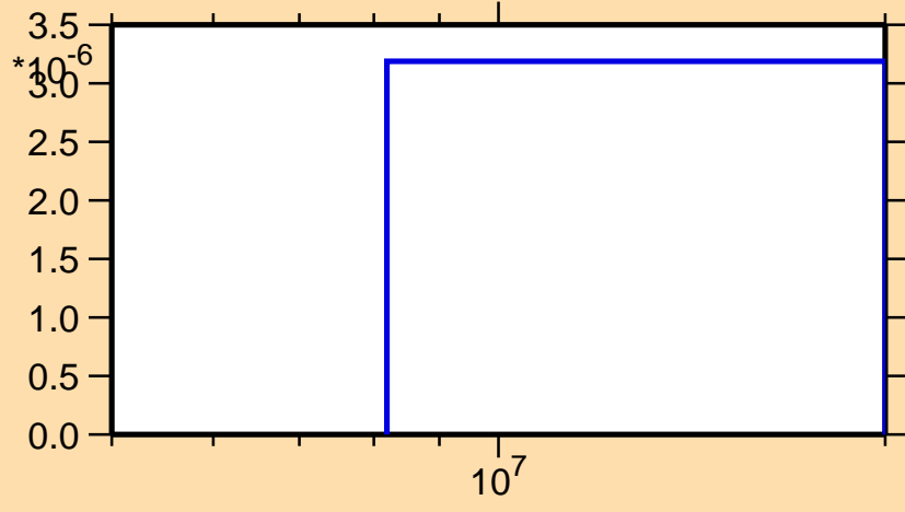
\sigma vs. E for ^{218}\text{At}(n,nd)
