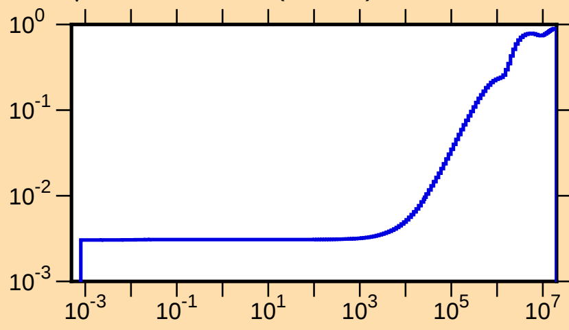
\mu vs. E for ^{221}\text{At}(\text{mt251})
