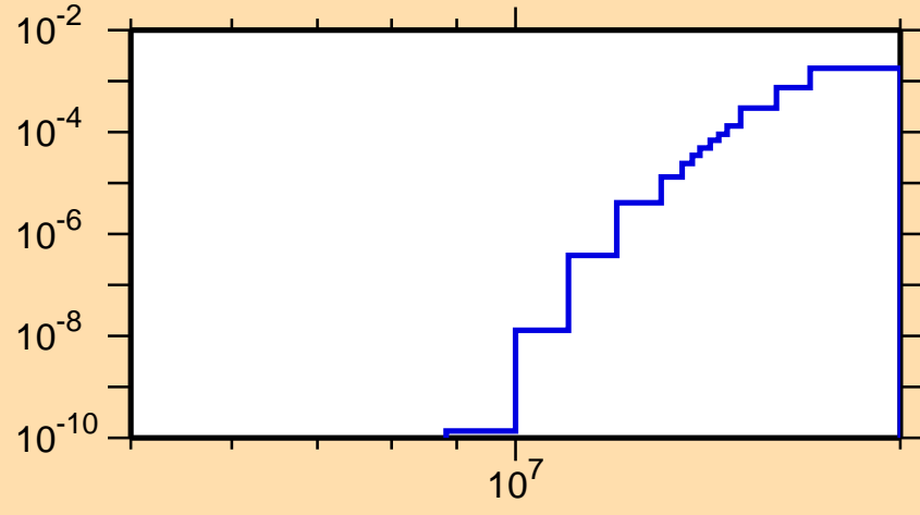
\sigma vs. E for ^{222}\text{At}(n,np)
