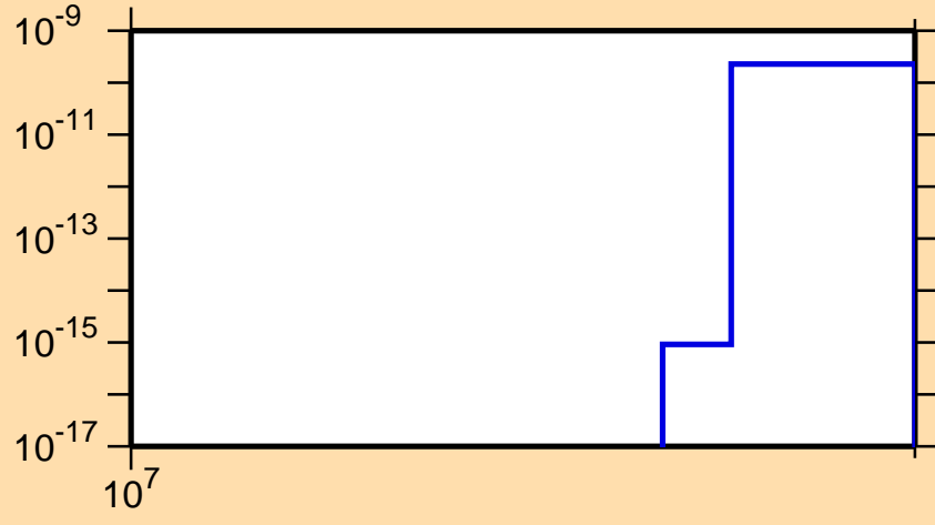
\sigma vs. E for ^{222}\text{At}(\text{mt } 42)
