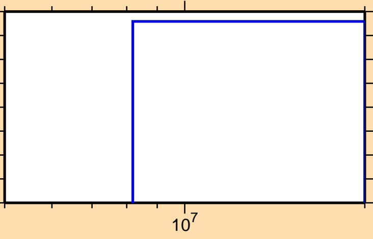
\sigma vs. E for ^{222}\text{At}(n,\text{He3})
