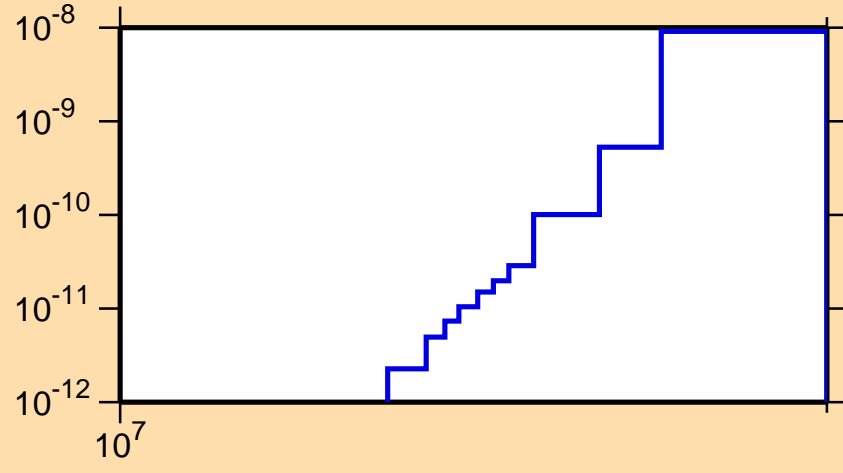
\sigma vs. E for ^{224}\text{At}(n,3n\alpha)
