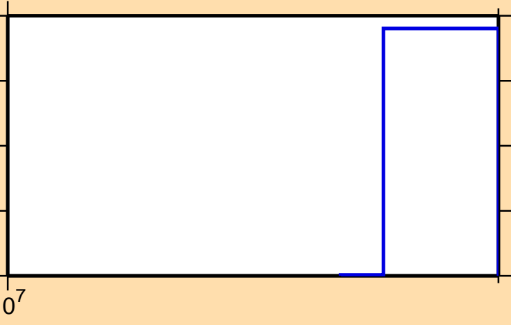
\sigma vs. E for ^{224}\text{At}(\text{mt } 11)
