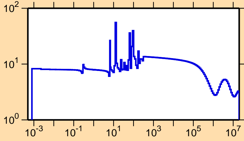
\sigma vs. E for ^{224}\text{At}(n,\text{el.})
