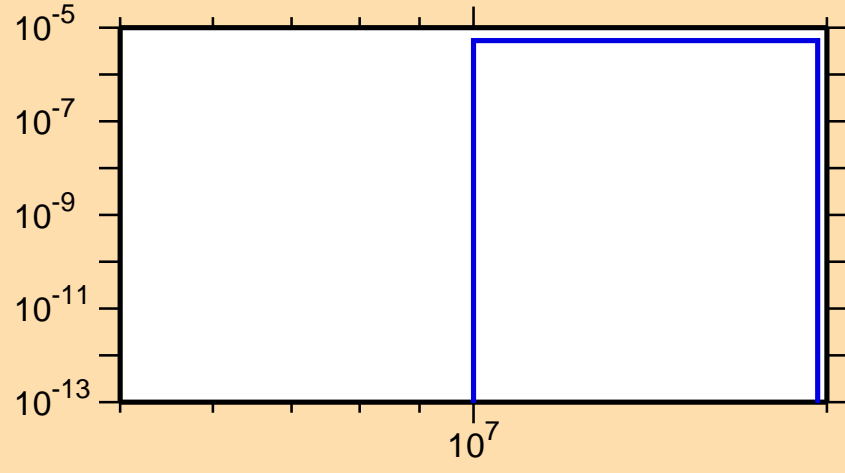
\sigma vs. E for ^{224}\text{At}(n,nt)
