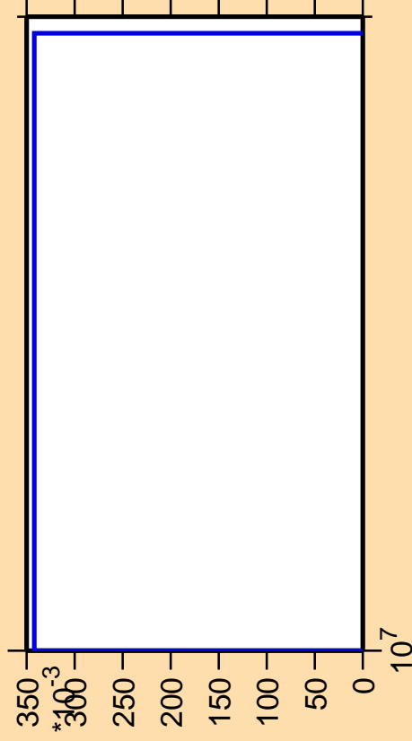
\Delta\sigma/\sigma vs. E for ^{224}\text{At}(\text{mt } 42)
