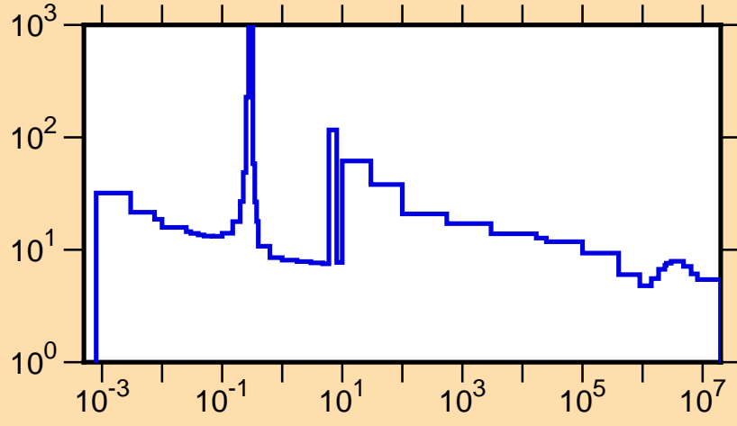
\sigma vs. E for ^{224}\text{At}(n,\text{tot.})
