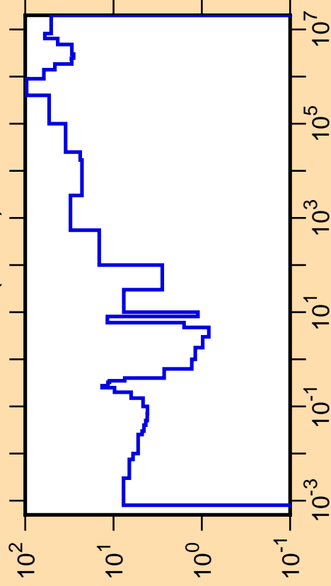
\Delta\sigma/\sigma vs. E for ^{224}\text{At}(n,\text{tot.})
