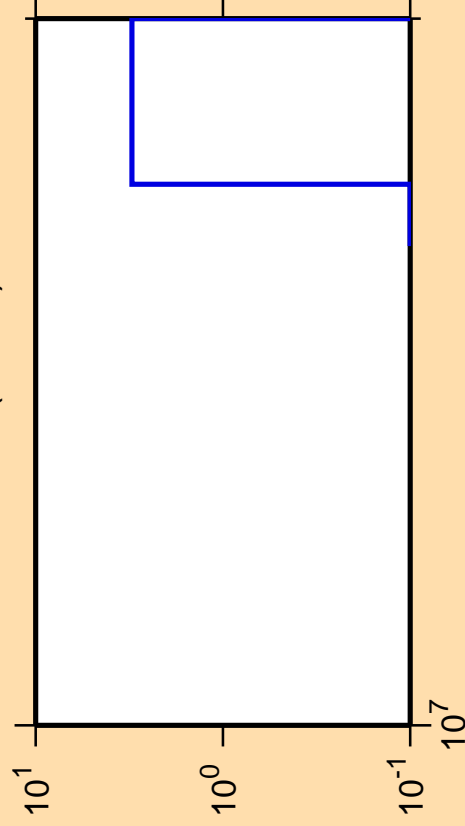
\Delta\sigma/\sigma vs. E for ^{227}\text{At} (mt 42)
