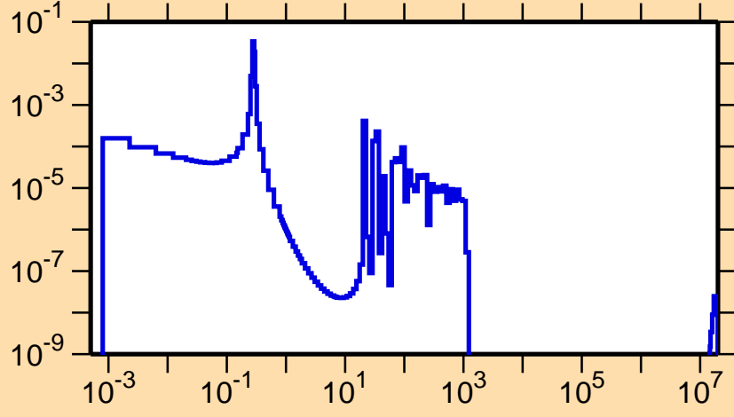
\sigma vs. E for ^{227}\text{At}(n,f)
