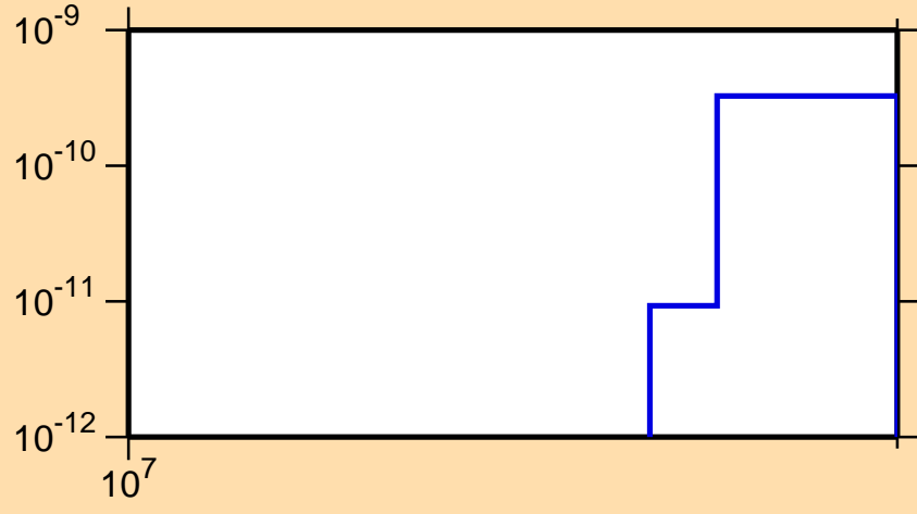
\sigma vs. E for ^{227}\text{At}(n,3n\alpha)
