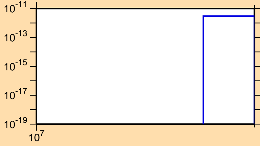
\sigma vs. E for ^{227}\text{At} (mt 42)
