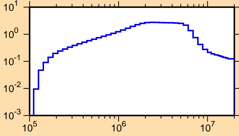
\sigma vs. E for ^{227}\text{At}(n,\text{inel.})
