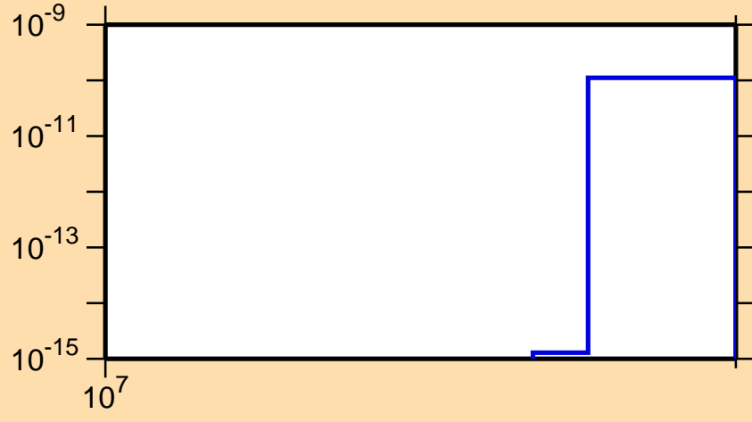
\sigma vs. E for ^{227}\text{At}(\text{mt } 11)
