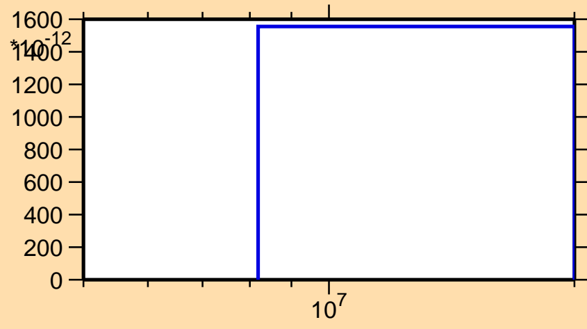
\sigma vs. E for ^{227}\text{At}(n,2np)
