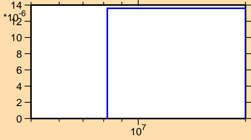
\sigma vs. E for ^{227}\text{At}(n,np)
