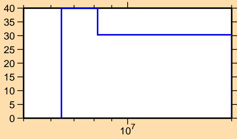
\Delta\sigma/\sigma vs. E for ^{227}\text{At}(n,el.)
