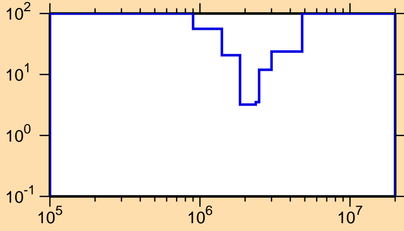
\Delta\sigma/\sigma vs. E for ^{227}\text{At}(n,n\text{cont.})
