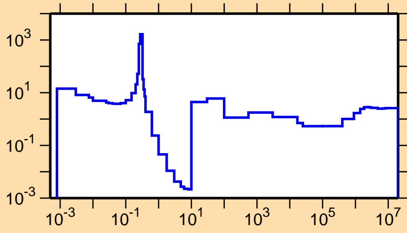
\sigma vs. E for ^{227}\text{At}(n,\text{nonel.})
