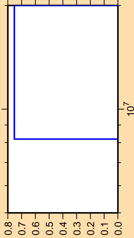
\Delta\sigma/\sigma vs. E for ^{227}\text{At}(\text{mt } 11)
