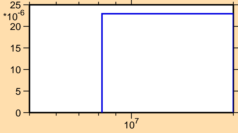
\sigma vs. E for ^{227}\text{At}(n,d)
