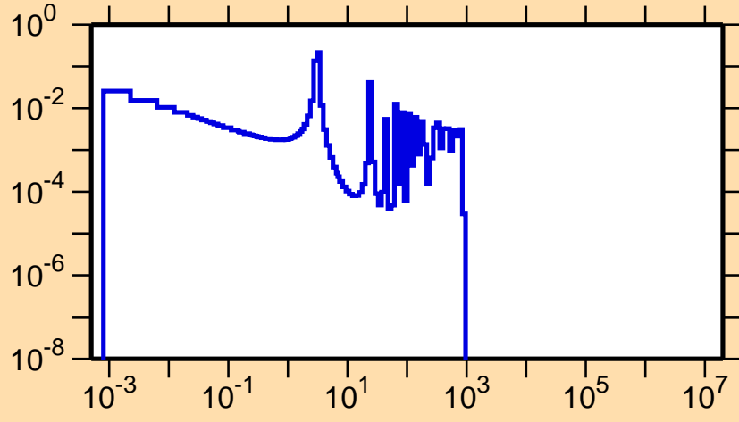
\sigma vs. E for ^{228}\text{At}(n,f)
