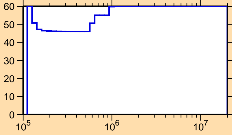
\Delta\sigma/\sigma vs. E for ^{228}\text{At}(n,n_1)
