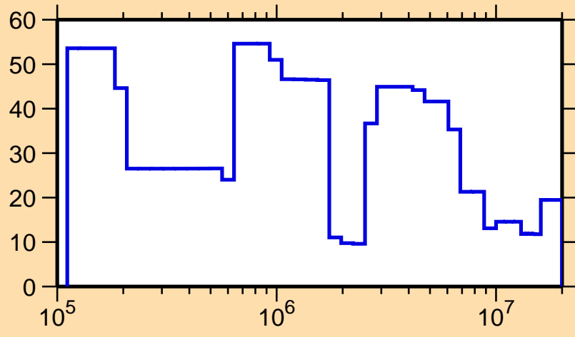
\Delta\sigma/\sigma vs. E for ^{228}\text{At}(n,\text{el.})
