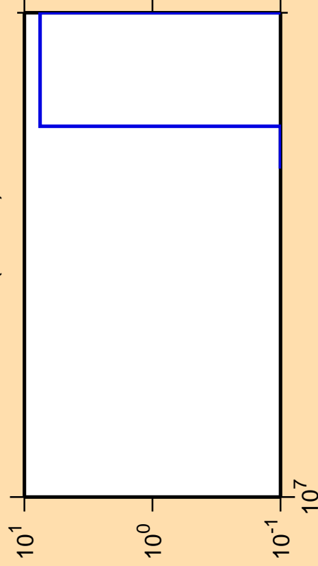
\Delta\sigma/\sigma vs. E for ^{228}\text{At} (mt 42)
