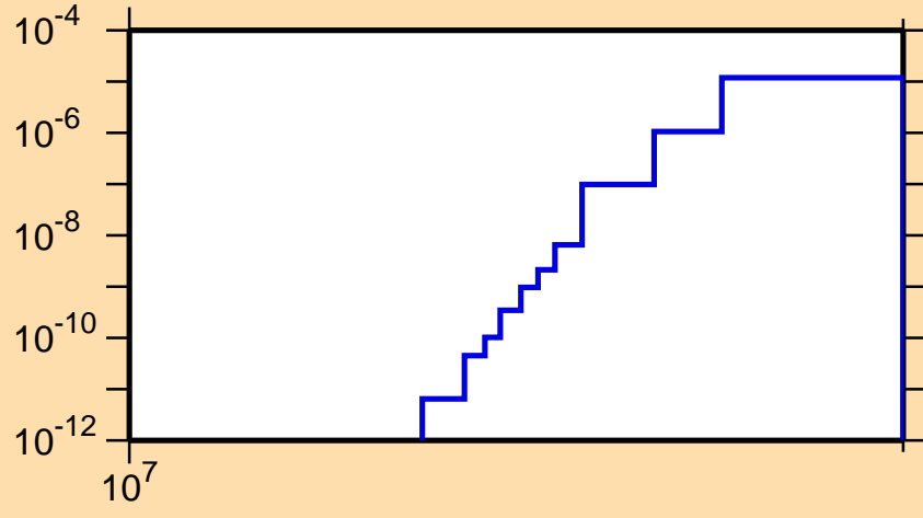
\sigma vs. E for ^{228}\text{At}(n,\text{nd})
