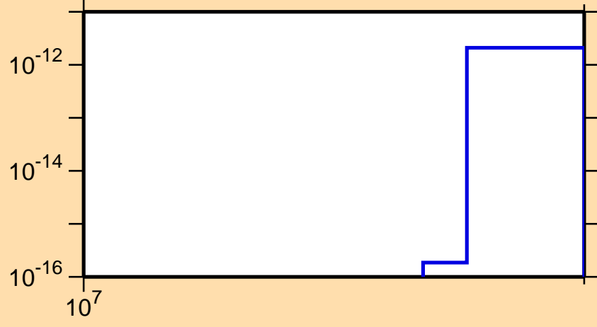
\sigma vs. E for ^{228}\text{At} (mt 42)
