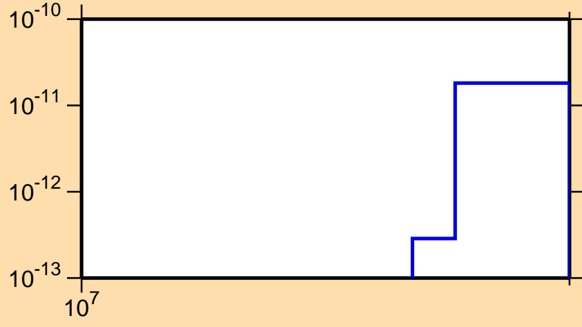
\sigma vs. E for ^{228}\text{At}(n,3n\alpha)
