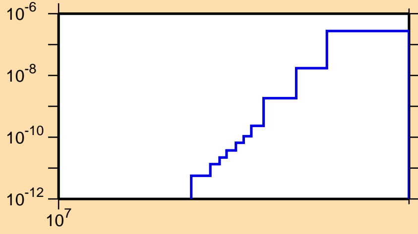
\sigma vs. E for ^{228}\text{At}(n,2n\alpha)
