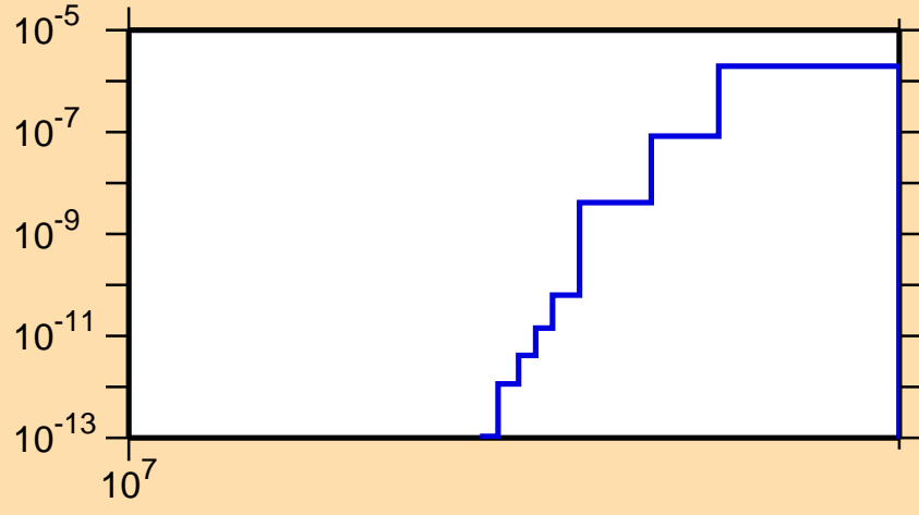
\sigma vs. E for ^{228}\text{At}(n,2np)
