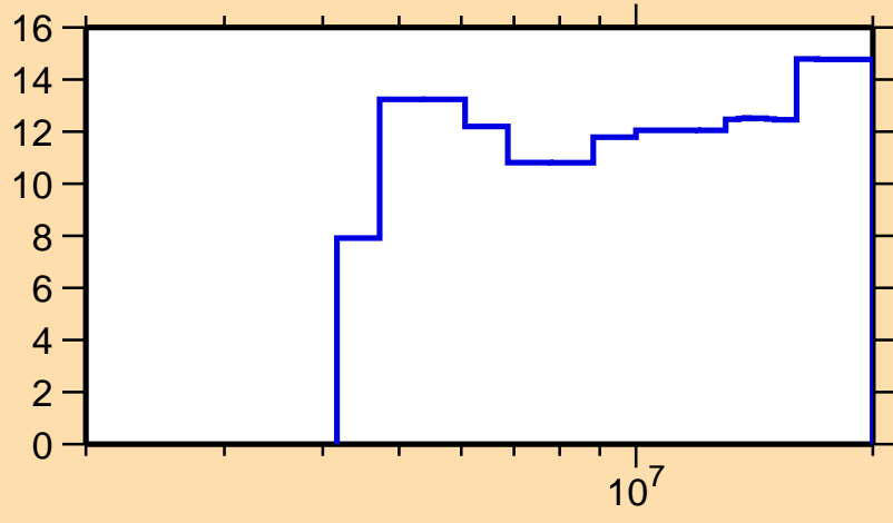
\Delta\sigma/\sigma vs. E for ^{228}\text{At}(n,\text{nonel.})
