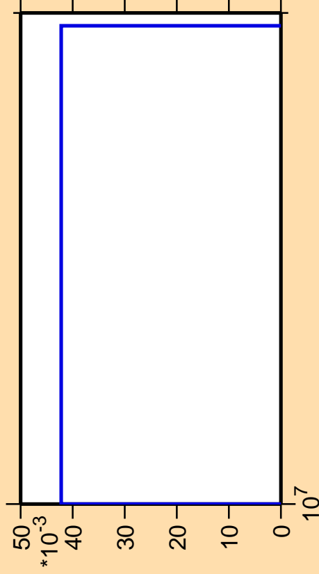
\Delta\sigma/\sigma vs. E for ^{228}\text{At} (mt 42)
