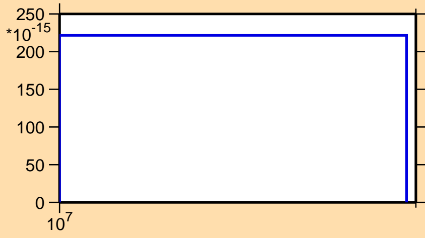
\sigma vs. E for ^{228}\text{At}(\text{mt } 11)
