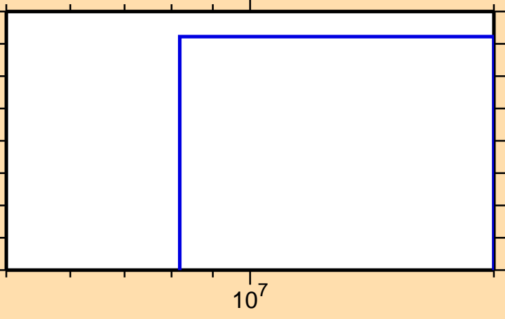
\sigma vs. E for ^{228}\text{At}(n,d)
