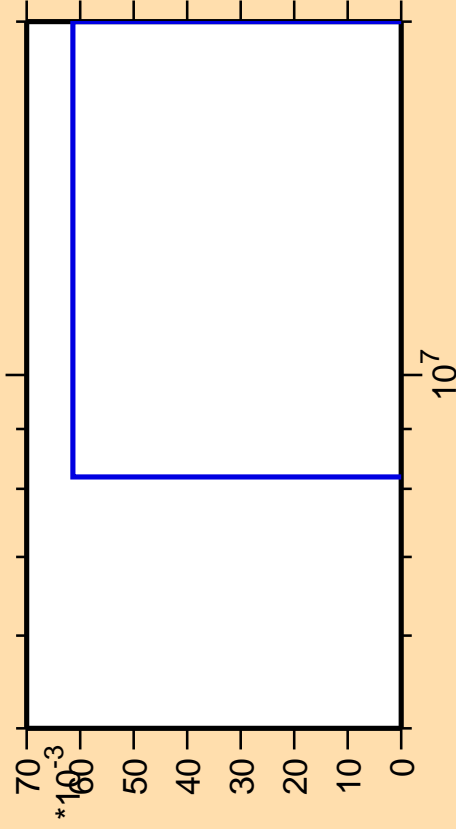
\Delta\sigma/\sigma vs. E for ^{228}\text{At}(\text{mt } 42)
