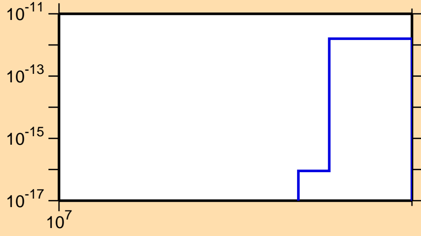
\sigma vs. E for ^{229}\text{At}(\text{mt } 42)
