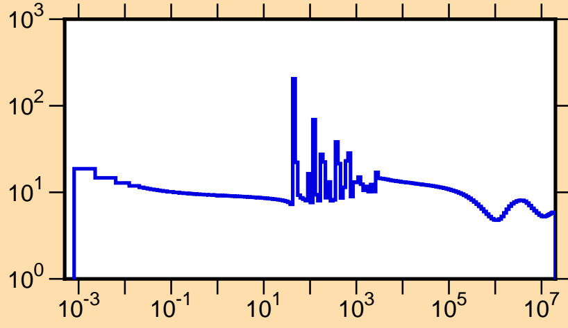
\sigma vs. E for ^{229}\text{At}(n,\text{tot.})
