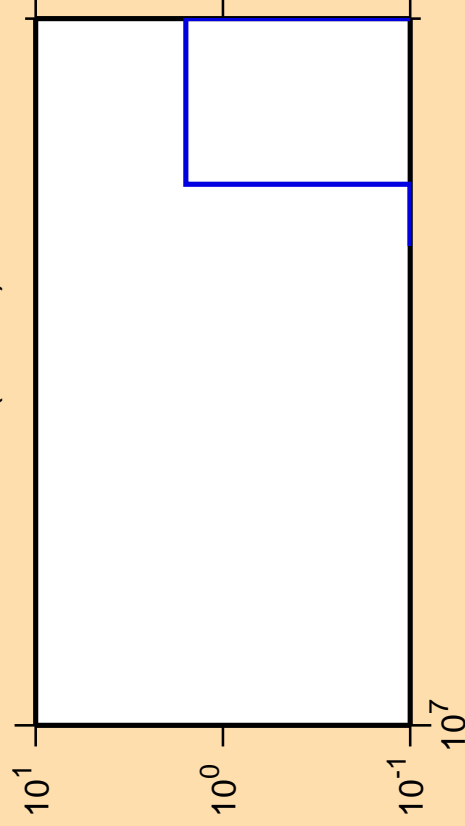
\Delta\sigma/\sigma vs. E for ^{229}\text{At}(\text{mt } 42)
