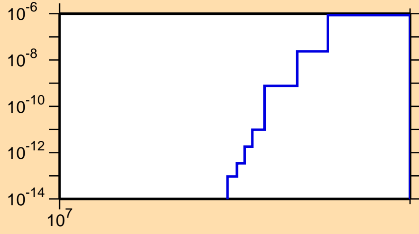
\sigma vs. E for ^{229}\text{At}(n,\text{nd})
