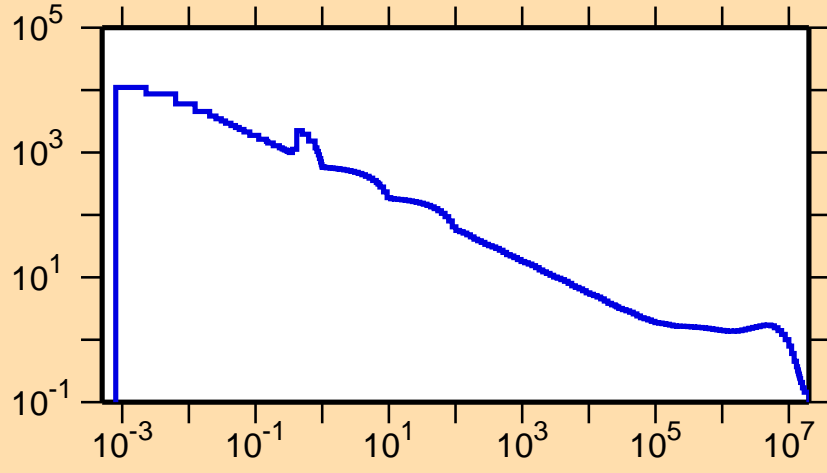
\sigma vs. E for ^{176}\text{Au}(n,p)
