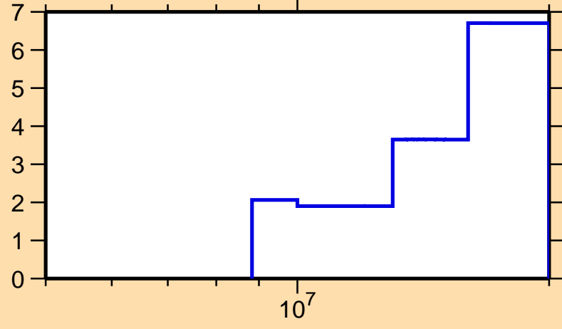
\Delta\sigma/\sigma vs. E for ^{176}\text{Au}(n,\text{tot.})
