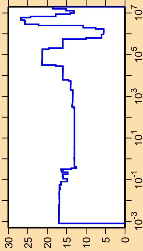
\Delta\sigma/\sigma vs. E for ^{176}\text{Au}(n,\text{el.})
