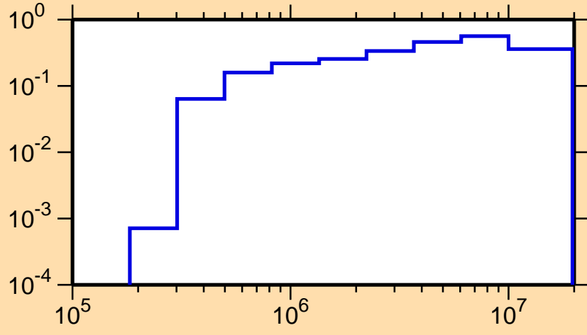
\sigma vs. E for ^{176}\text{Au}(n,\text{inel.})
