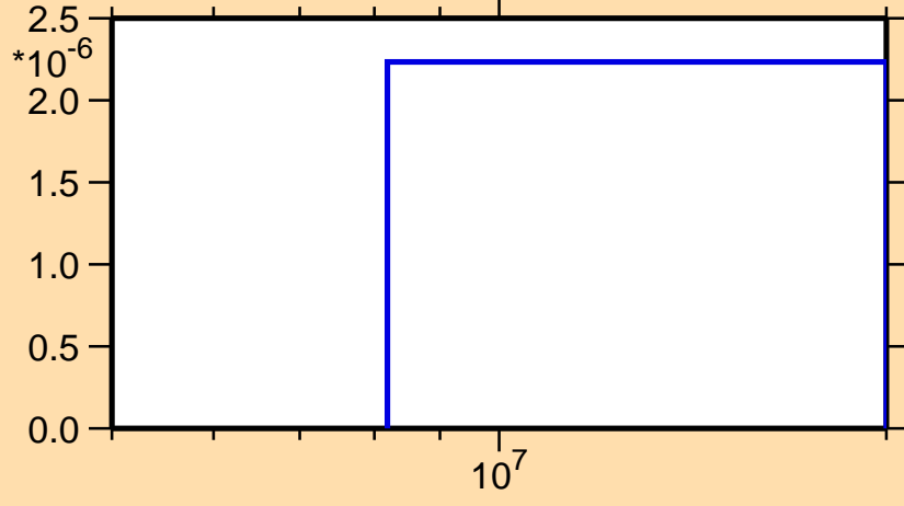
\sigma vs. E for ^{176}\text{Au}(n,nd)
