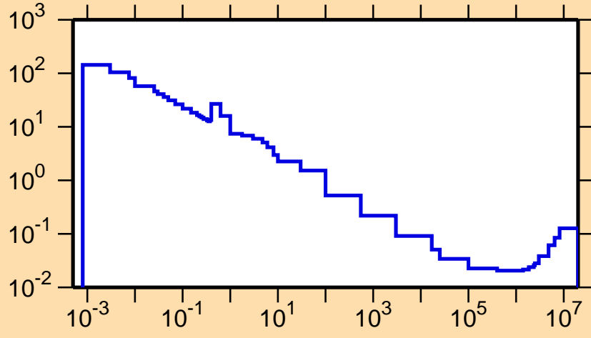
\sigma vs. E for ^{176}\text{Au}(n,\alpha)
