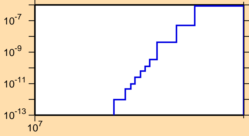
\sigma vs. E for ^{177}\text{Au}(n,pt)
