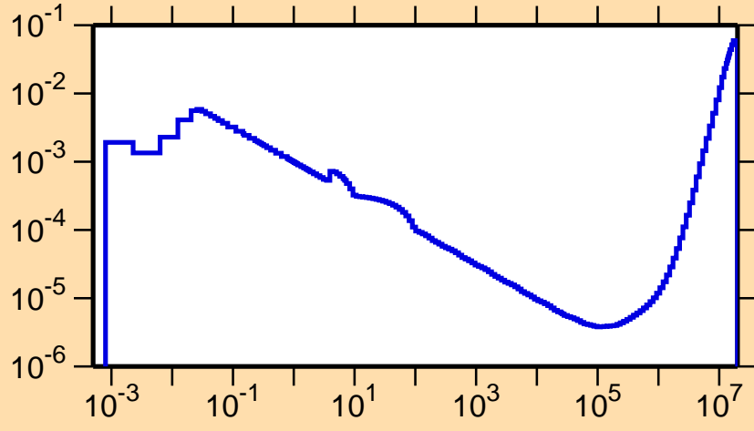
\sigma vs. E for ^{177}\text{Au}(n,p\alpha)
