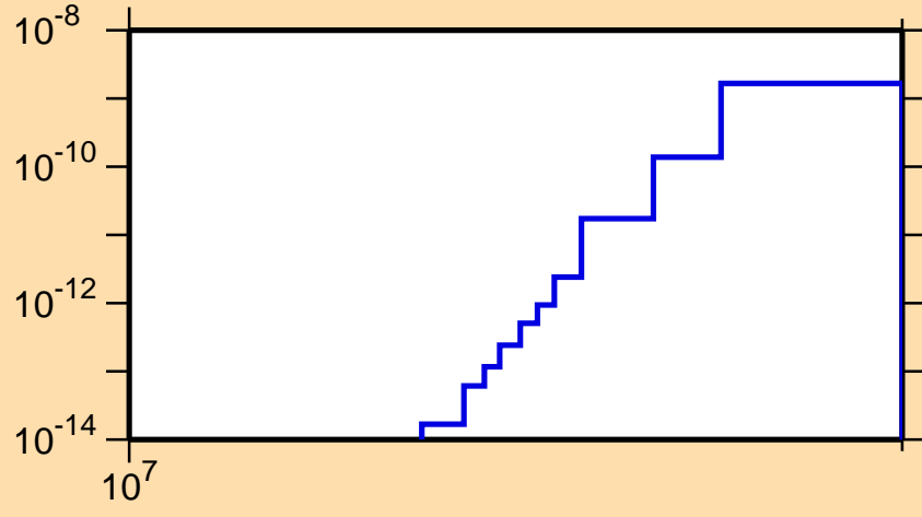
\sigma vs. E for ^{177}\text{Au}(\text{mt } 34)
