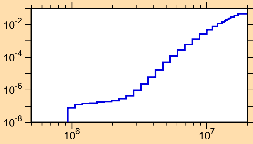
\sigma vs. E for ^{177}\text{Au}(n,n\alpha)
