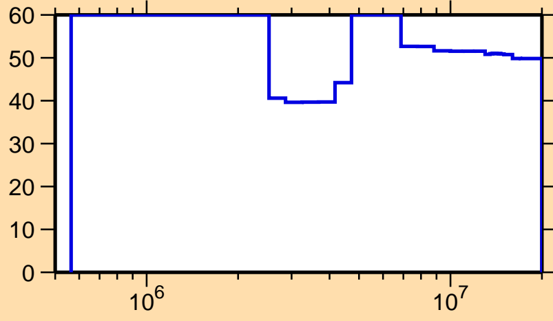
\Delta\sigma/\sigma vs. E for ^{177}\text{Au}(n,n_1)
