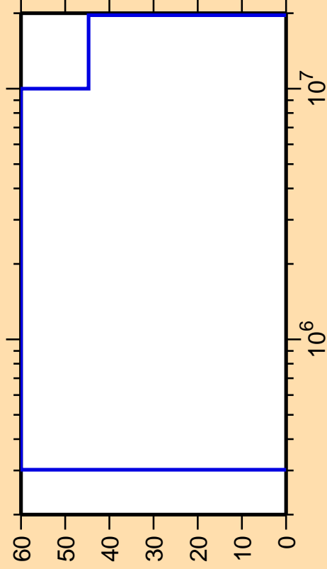
\Delta\sigma/\sigma vs. E for ^{177}\text{Au}(n,n_4)
