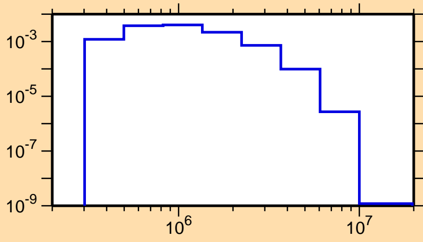
\sigma vs. E for ^{177}\text{Au}(n,n_4)
