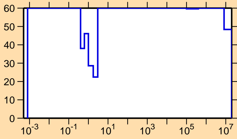
\Delta\sigma/\sigma vs. E for ^{177}\text{Au}(n,\gamma)
