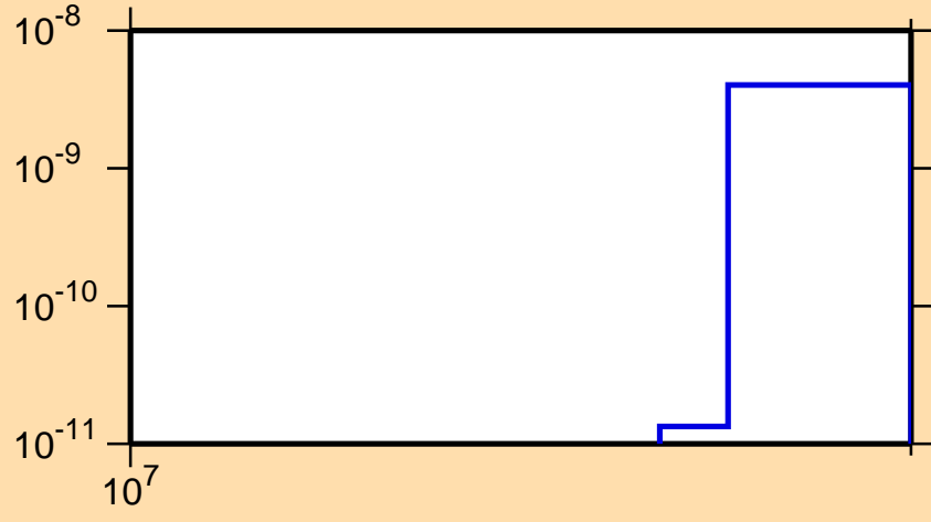
\sigma vs. E for ^{178}\text{Au}(n,nt)
