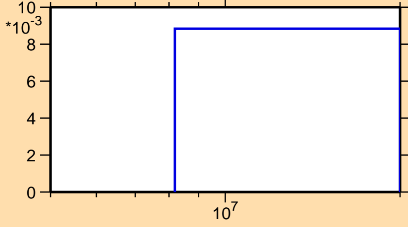
\sigma vs. E for ^{178}\text{Au}(n,2np)
