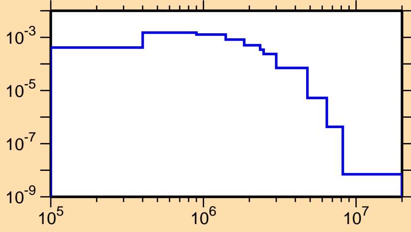
\sigma vs. E for ^{178}\text{Au}(n,n_1)
