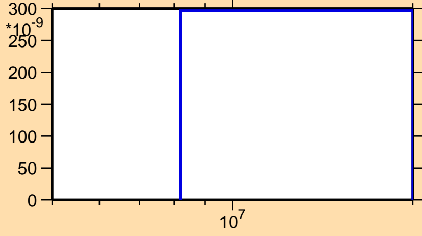
\sigma vs. E for ^{178}\text{Au}(n,\text{pt})
