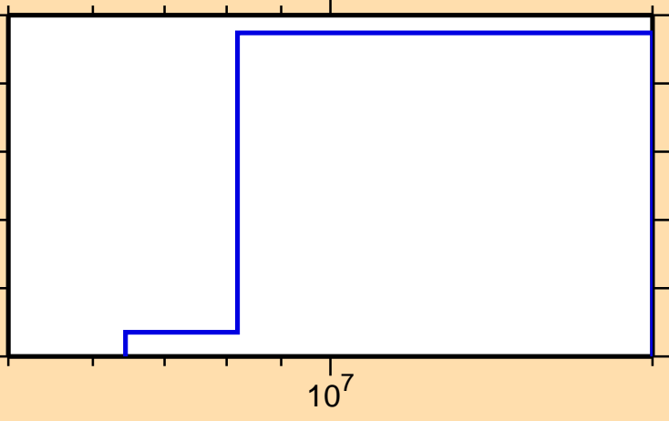
\sigma vs. E for ^{178}\text{Au}(\text{mt117})
