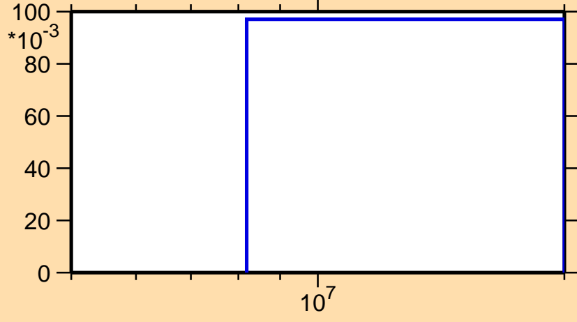
\sigma vs. E for ^{178}\text{Au}(n,2n)
