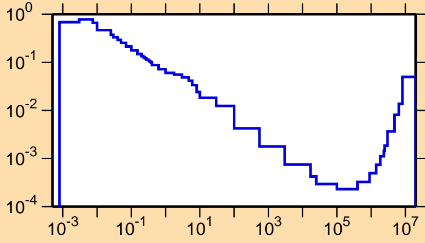
\sigma vs. E for ^{178}\text{Au}(n,p\alpha)
