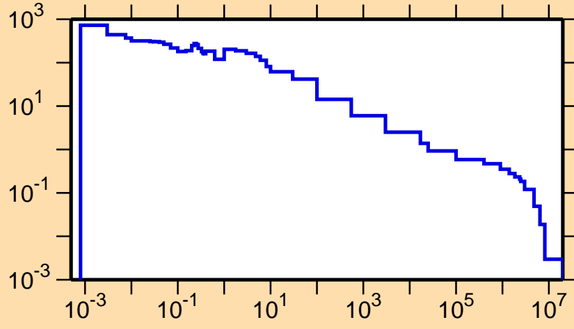
\sigma vs. E for ^{178}\text{Au}(n,\gamma)
