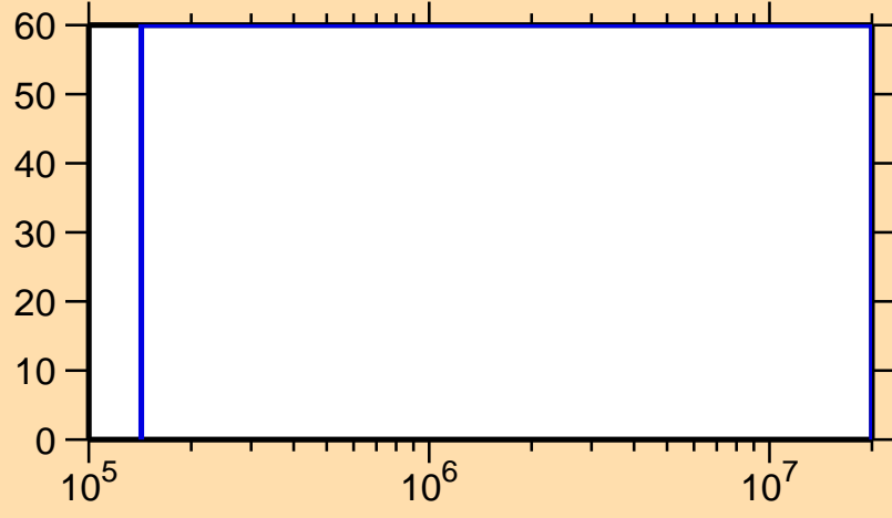
\Delta\sigma/\sigma vs. E for ^{179}\text{Au}(n,n\text{cont.})
