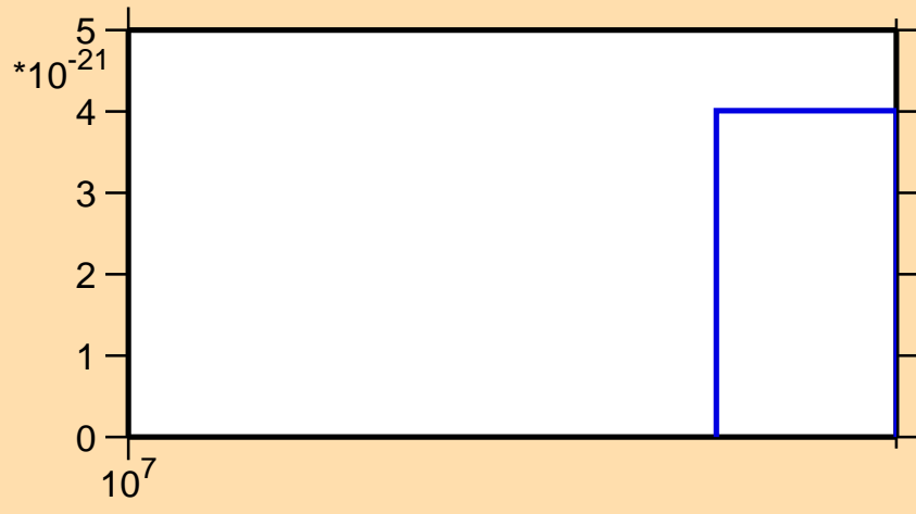
\sigma vs. E for ^{179}\text{Au} (mt 42)
