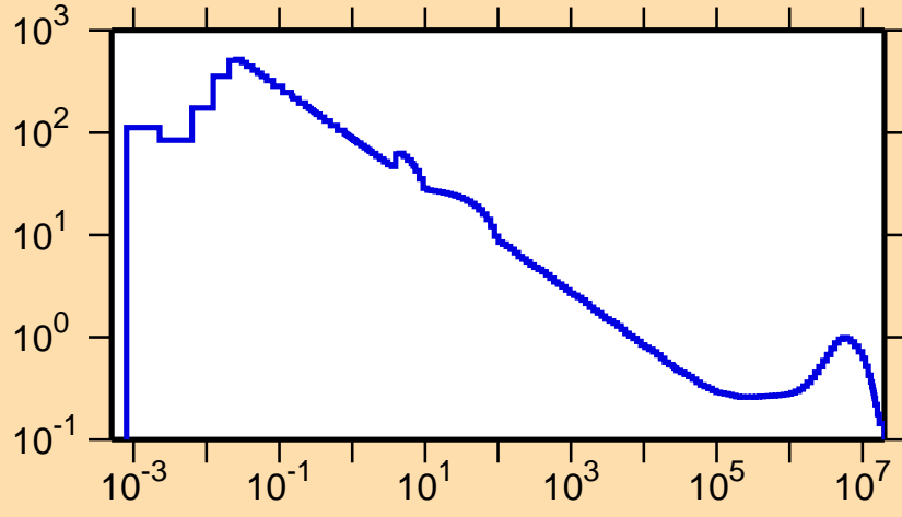
\sigma vs. E for ^{179}\text{Au}(n,p)
