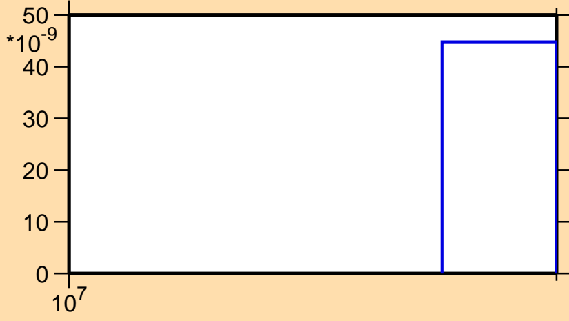
\sigma vs. E for ^{179}\text{Au}(n,3n)
