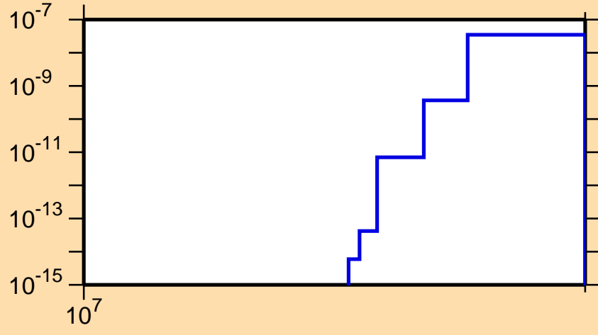
\sigma vs. E for ^{179}\text{Au}(n,nt)
