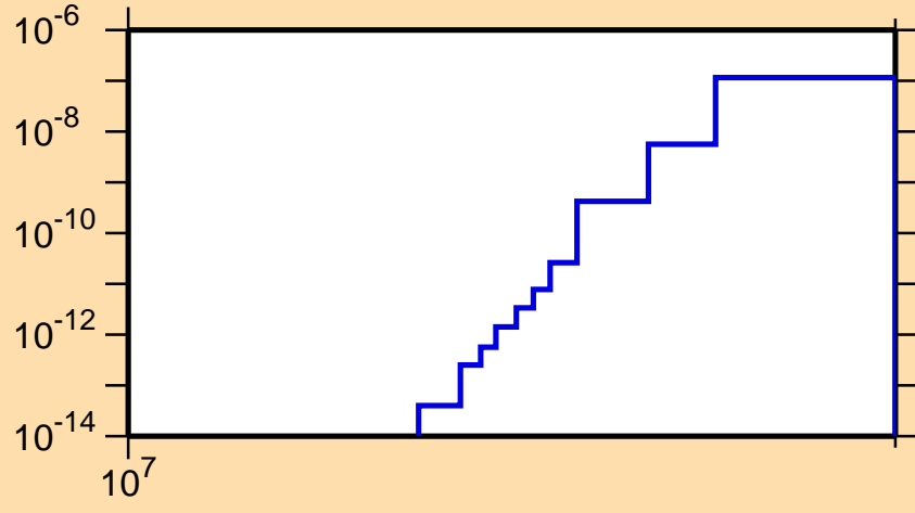
\sigma vs. E for ^{179}\text{Au}(n,pt)
