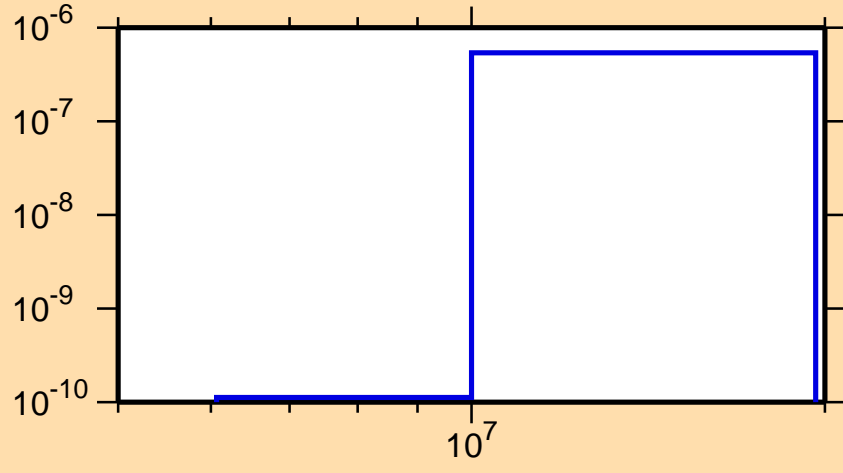
\sigma vs. E for ^{179}\text{Au}(\text{mt117})
