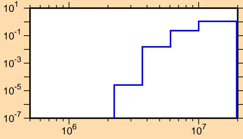
\sigma vs. E for ^{179}\text{Au}(n,np)
