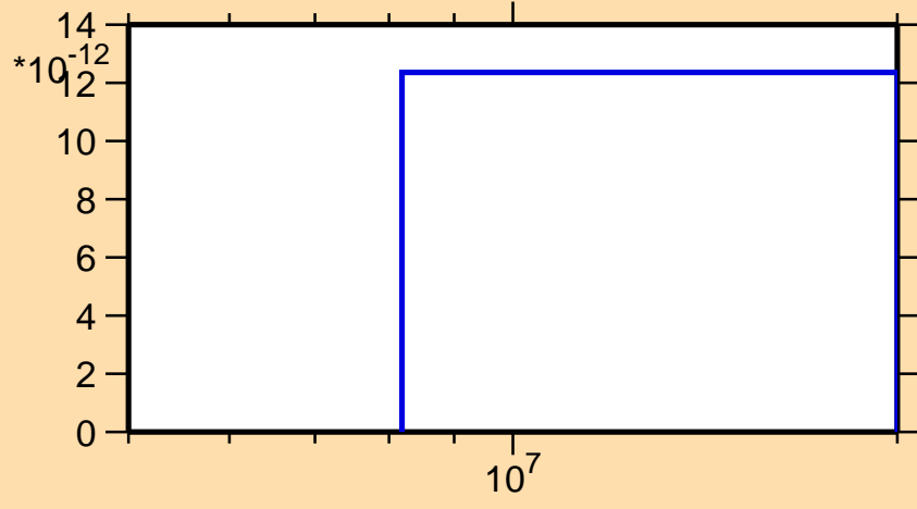
\sigma vs. E for ^{179}\text{Au}(\text{mt } 34)
