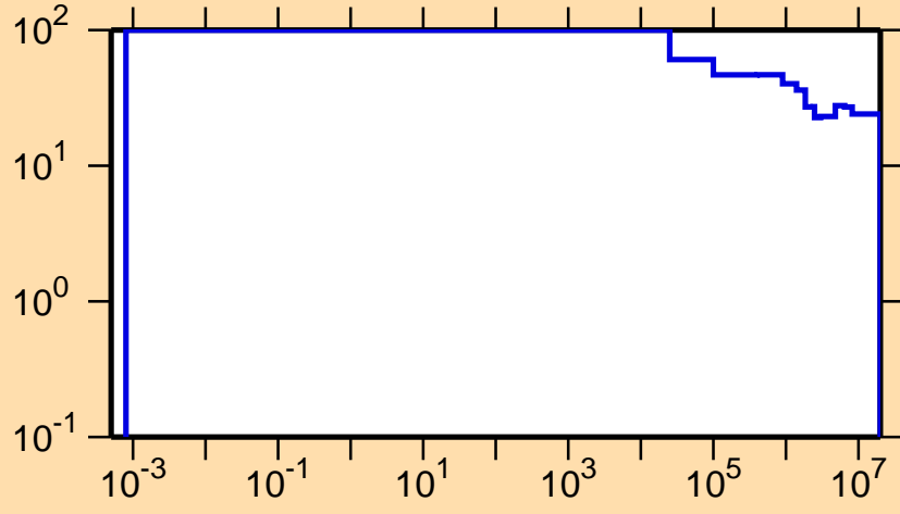
\Delta\sigma/\sigma vs. E for ^{179}\text{Au}(n,\text{nonel.})
