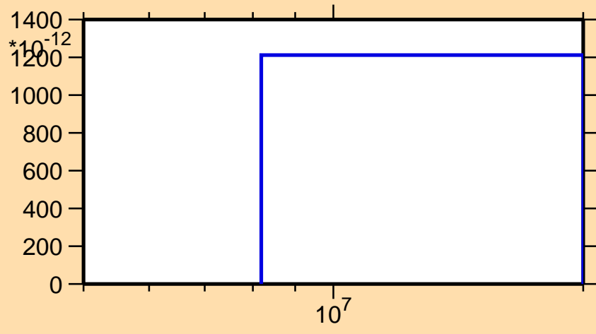
\sigma vs. E for ^{179}\text{Au}(n,\text{pt})
