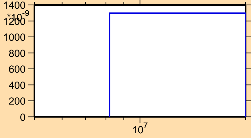
\sigma vs. E for ^{179}\text{Au}(n,\text{pd})
