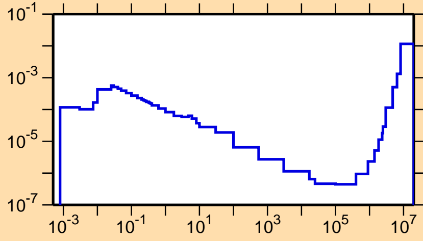
\sigma vs. E for ^{179}\text{Au}(n,p\alpha)
