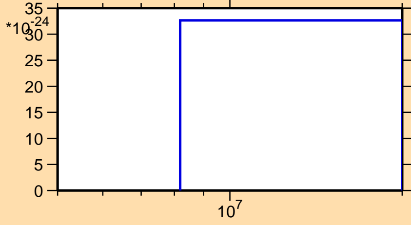
\sigma vs. E for ^{179}\text{Au}(\text{mt } 42)
