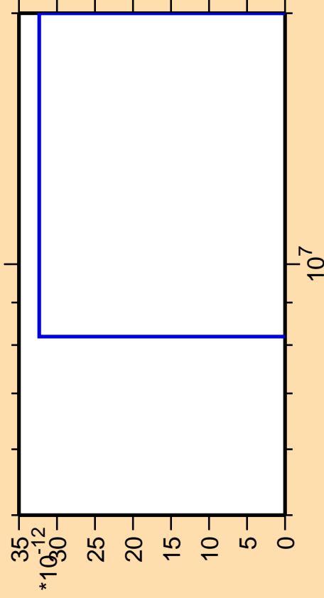
\Delta\sigma/\sigma vs. E for ^{179}\text{Au}(\text{mt } 42)
