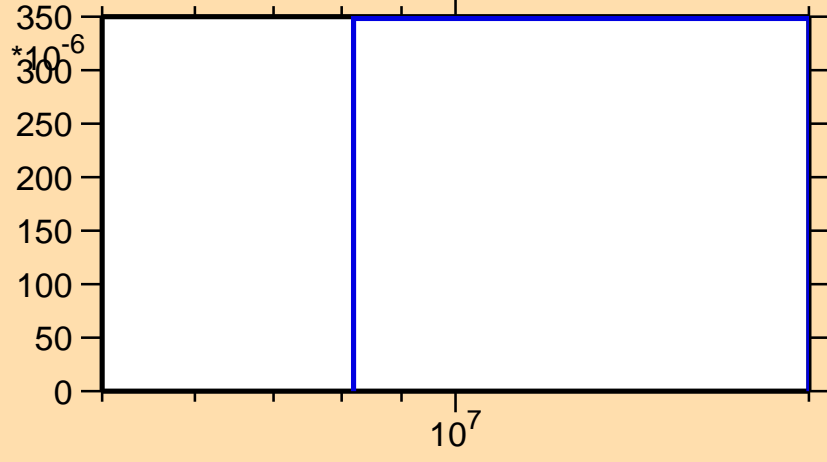
\sigma vs. E for ^{179}\text{Au}(n,2np)
