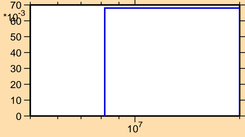
\sigma vs. E for ^{179}\text{Au}(n,2n)
