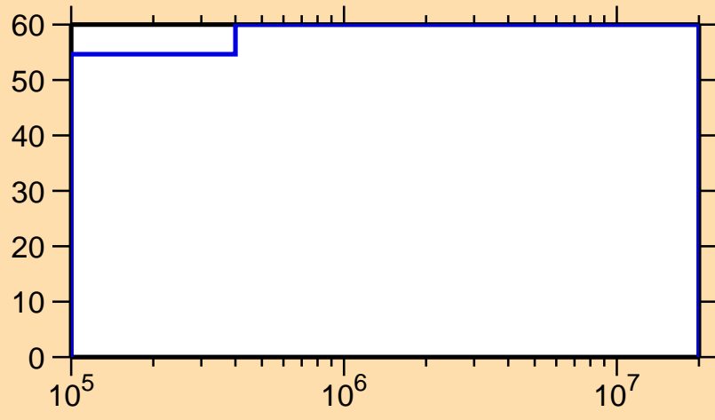
\Delta\sigma/\sigma vs. E for ^{179}\text{Au}(n,n_1)
