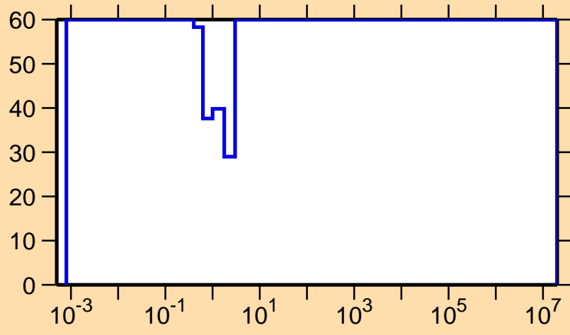
\Delta\sigma/\sigma vs. E for ^{179}\text{Au}(n,\gamma)
