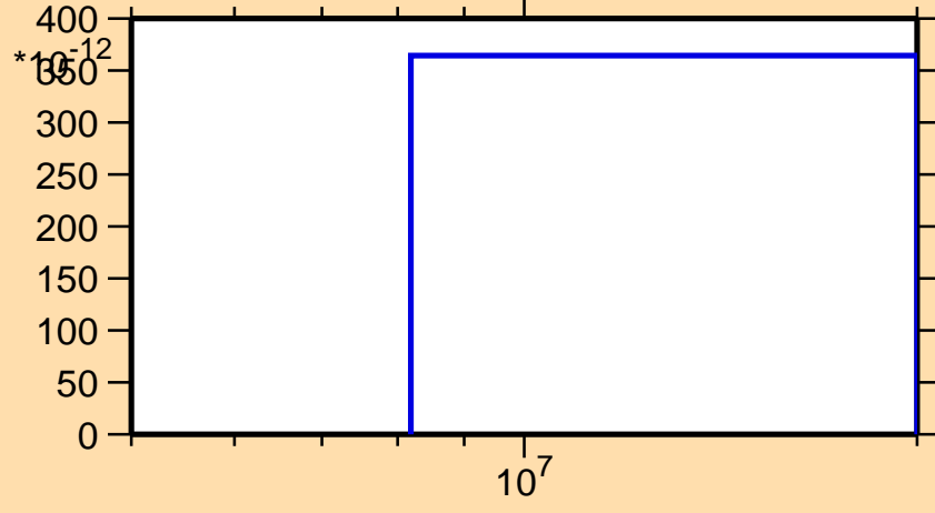
\sigma vs. E for ^{179}\text{Au}(n,3n)
