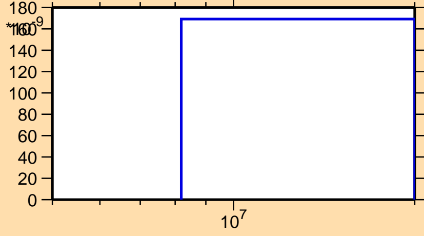
\sigma vs. E for ^{179}\text{Au}(n,nd)
