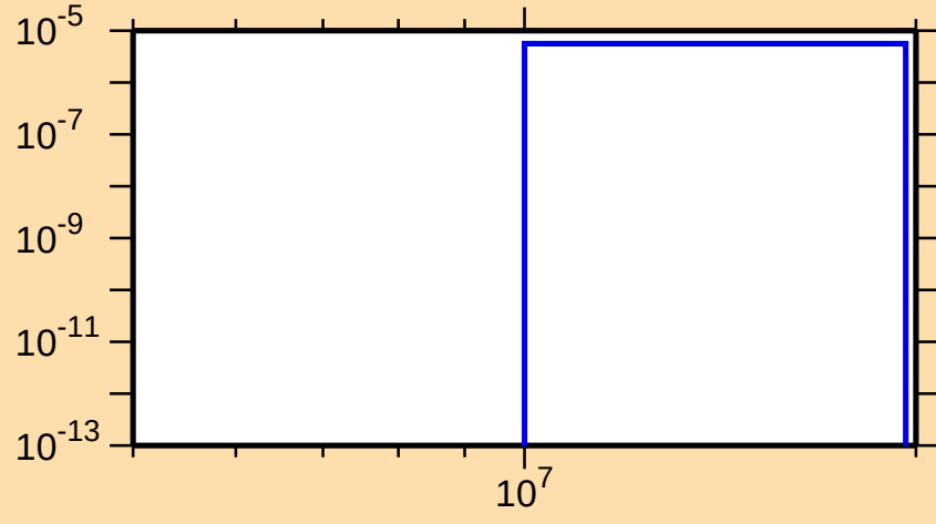
\sigma vs. E for ^{180}\text{Au}(n,nd)
