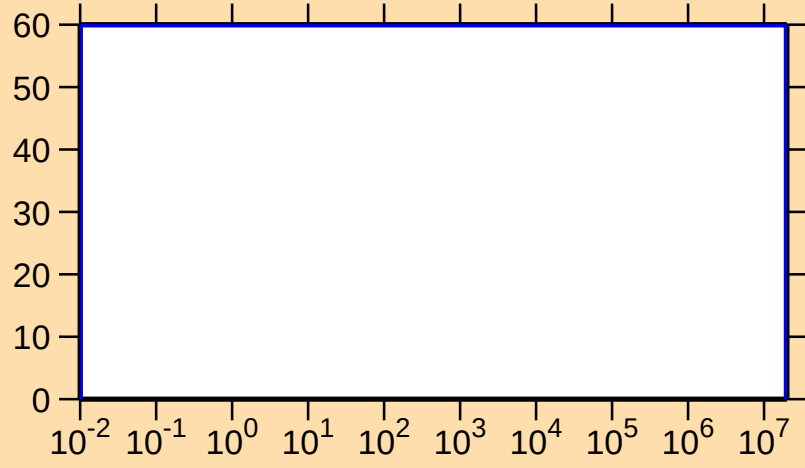
\Delta\sigma/\sigma vs. E for ^{180}\text{Au}(n,p)
