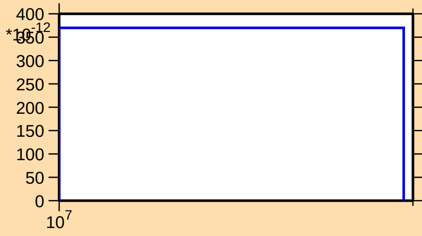
\sigma vs. E for ^{180}\text{Au}(\text{mt } 34)
