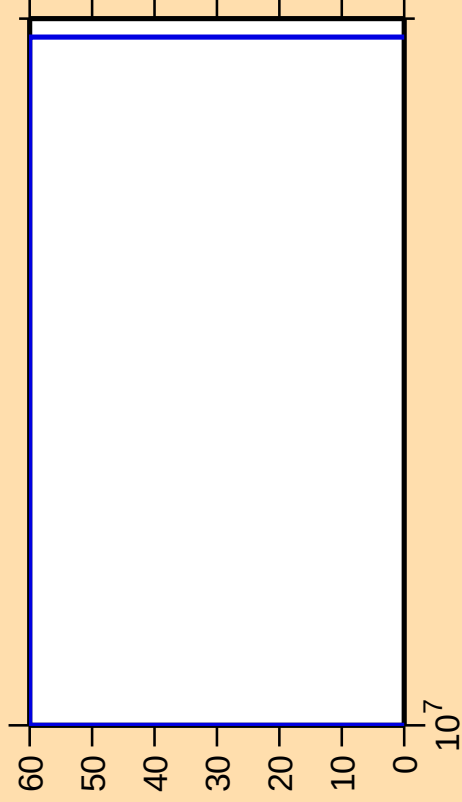
\Delta\sigma/\sigma vs. E for ^{180}\text{Au}(\text{mt } 34)
