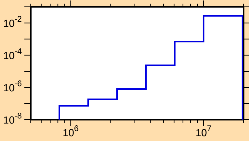
\sigma vs. E for ^{180}\text{Au}(n,n\alpha)
