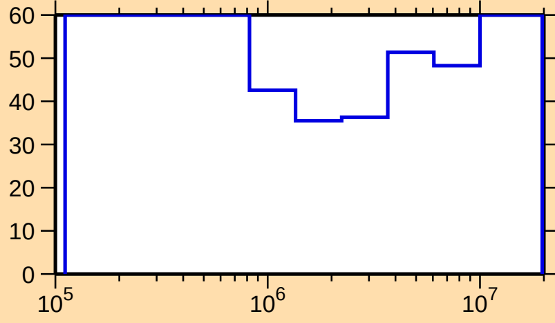
\Delta\sigma/\sigma vs. E for ^{180}\text{Au}(n,n_1)
