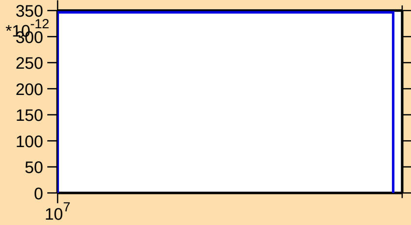
\sigma vs. E for ^{180}\text{Au}(n,3n\alpha)
