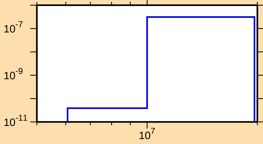
\sigma vs. E for ^{180}\text{Au}(\text{mt117})
