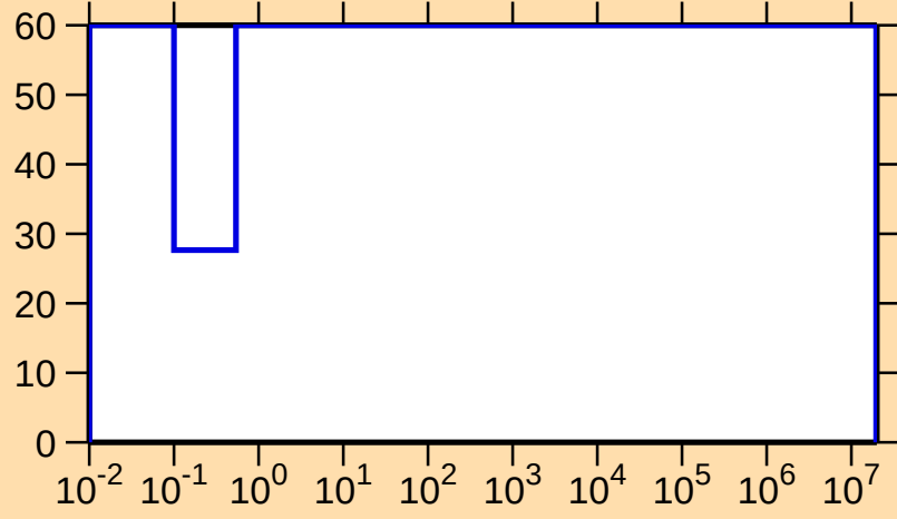
\Delta\sigma/\sigma vs. E for ^{180}\text{Au}(n,\gamma)
