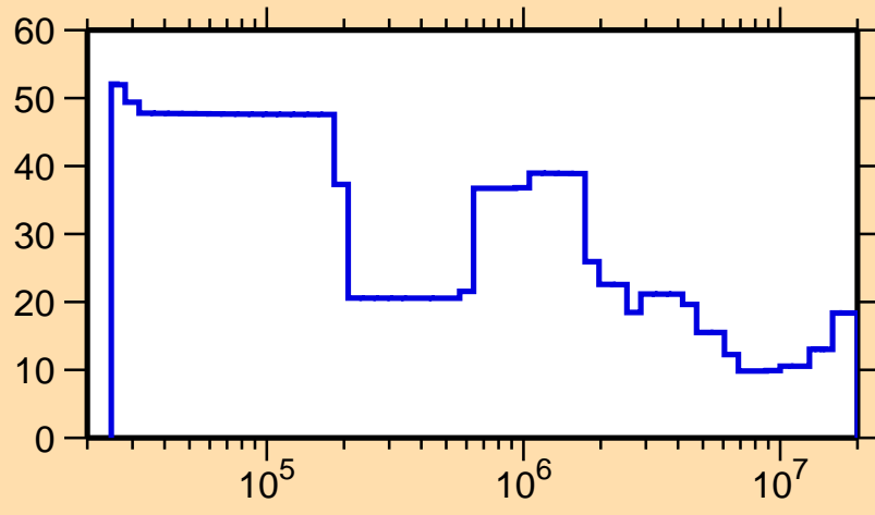
\Delta\sigma/\sigma vs. E for ^{182}\text{Au}(n,\text{tot.})
