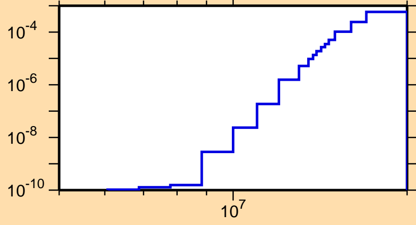
\sigma vs. E for ^{182}\text{Au}(n,2n\alpha)
