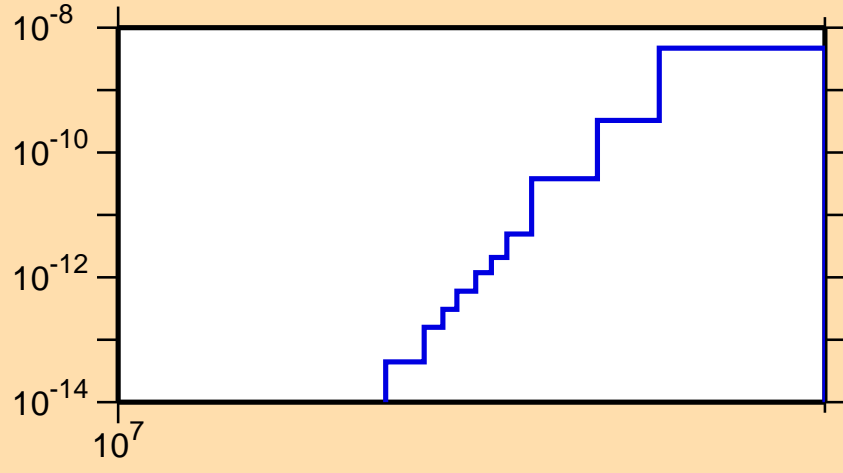
\sigma vs. E for ^{182}\text{Au}(\text{mt } 34)
