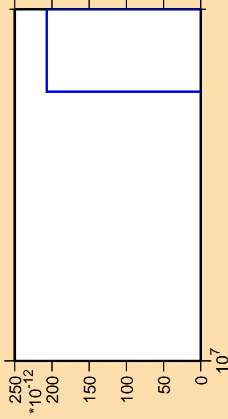
\Delta\sigma/\sigma vs. E for ^{182}\text{Au} (mt 42)
