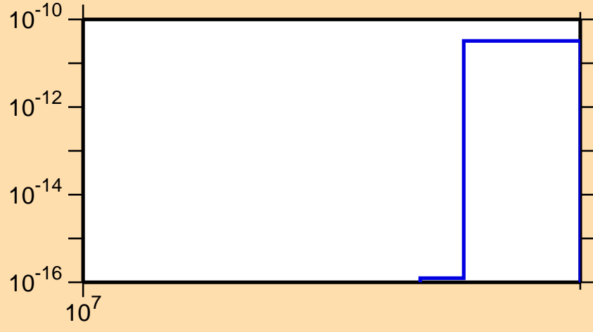
\sigma vs. E for ^{182}\text{Au}(n,3n\alpha)
