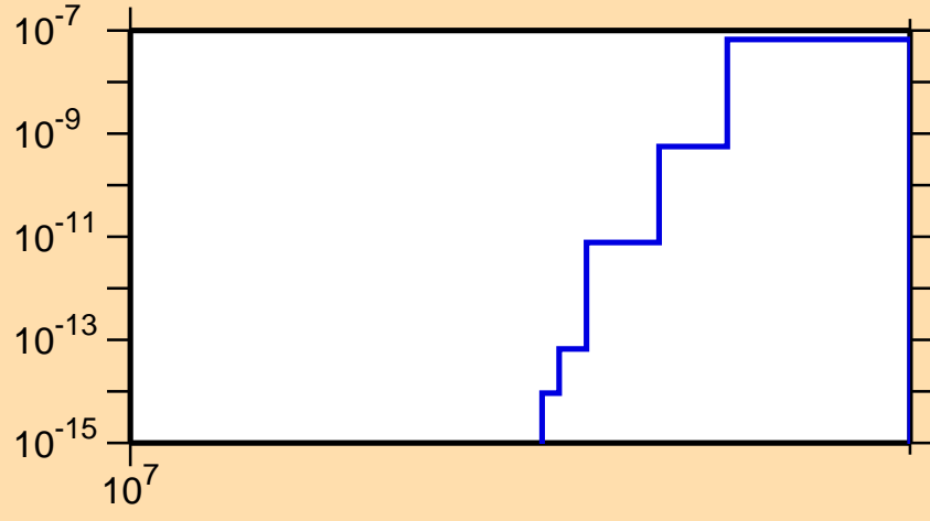
\sigma vs. E for ^{182}\text{Au}(n,nt)
