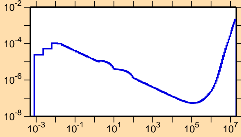
\sigma vs. E for ^{182}\text{Au}(n,p\alpha)
