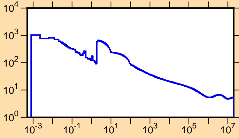
\sigma vs. E for ^{182}\text{Au}(n,\text{tot.})
