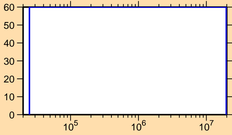
\Delta\sigma/\sigma vs. E for ^{182}\text{Au}(n,n_1)
