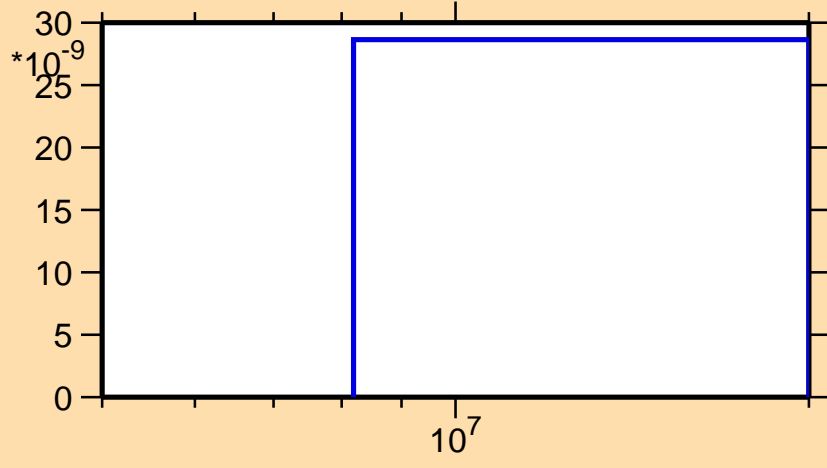
\sigma vs. E for ^{182}\text{Au}(\text{mt117})
