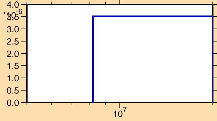
\sigma vs. E for ^{182}\text{Au}(n,nd)
