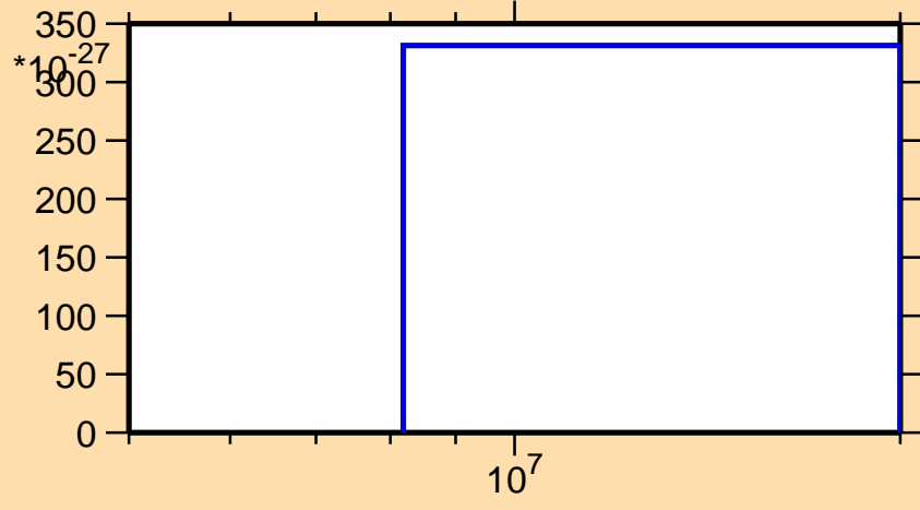
\sigma vs. E for ^{182}\text{Au}(\text{mt } 42)
