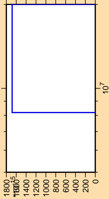
\Delta\sigma/\sigma vs. E for ^{182}\text{Au}(\text{mt } 42)
