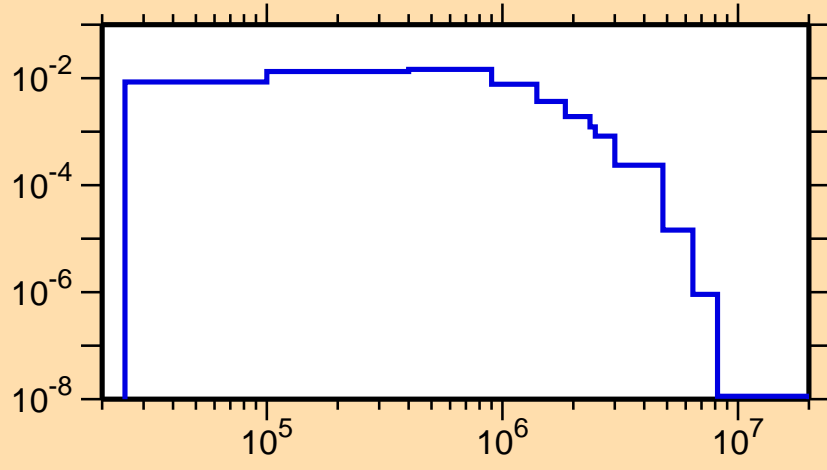
\sigma vs. E for ^{182}\text{Au}(n,n_1)
