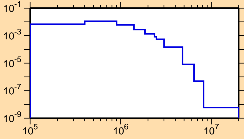
\sigma vs. E for ^{182}\text{Au}(n,n_3)
