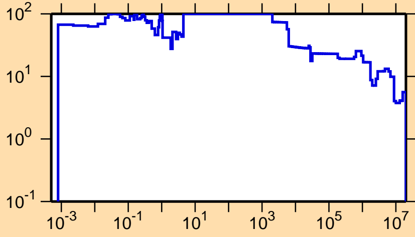
\Delta\sigma/\sigma vs. E for ^{183}\text{Au}(n,\text{tot.})
