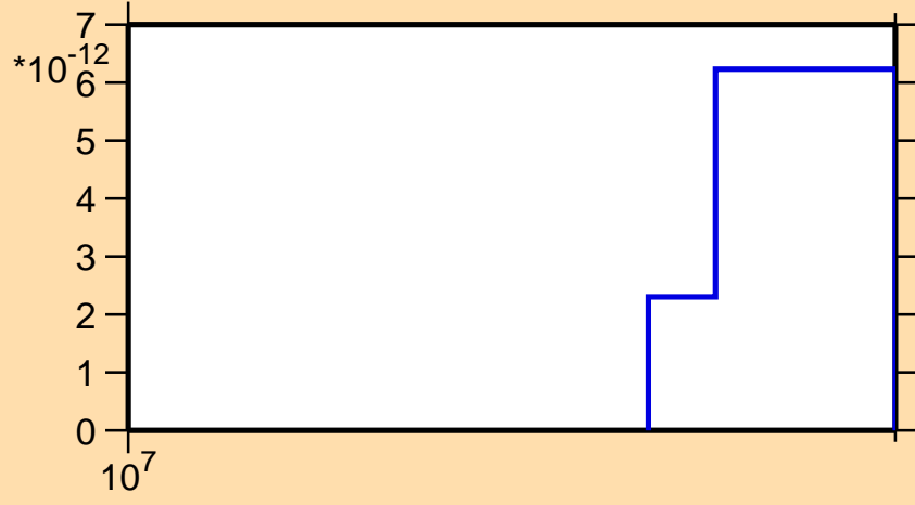
\sigma vs. E for ^{183}\text{Au}(n,3n\alpha)
