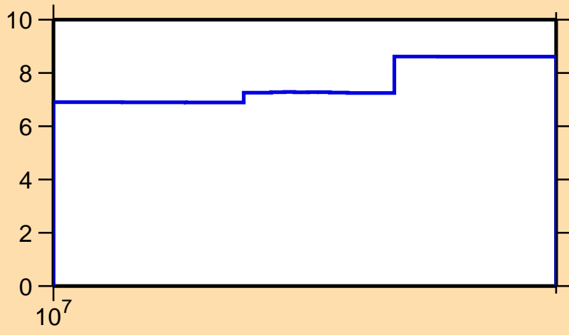
\Delta\sigma/\sigma vs. E for ^{183}\text{Au}(n,\text{el.})
