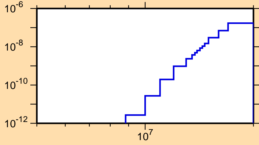
\sigma vs. E for ^{183}\text{Au}(\text{mt117})
