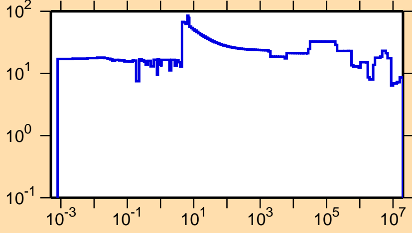
\Delta\sigma/\sigma vs. E for ^{183}\text{Au}(n,\text{el.})
