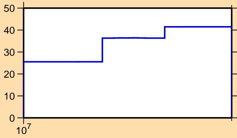
\Delta\sigma/\sigma vs. E for ^{183}\text{Au}(n,\text{inel.})
