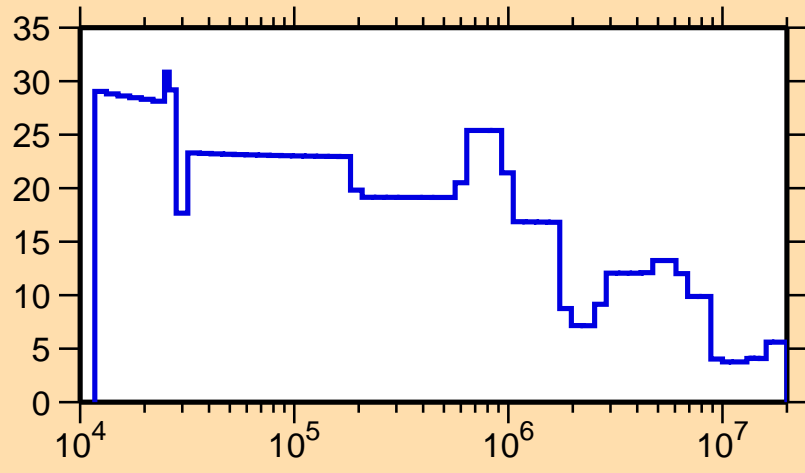
\Delta\sigma/\sigma vs. E for ^{183}\text{Au}(n,\text{tot.})
