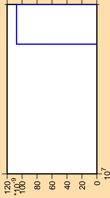
\Delta\sigma/\sigma vs. E for ^{183}\text{Au}(\text{mt } 42)
