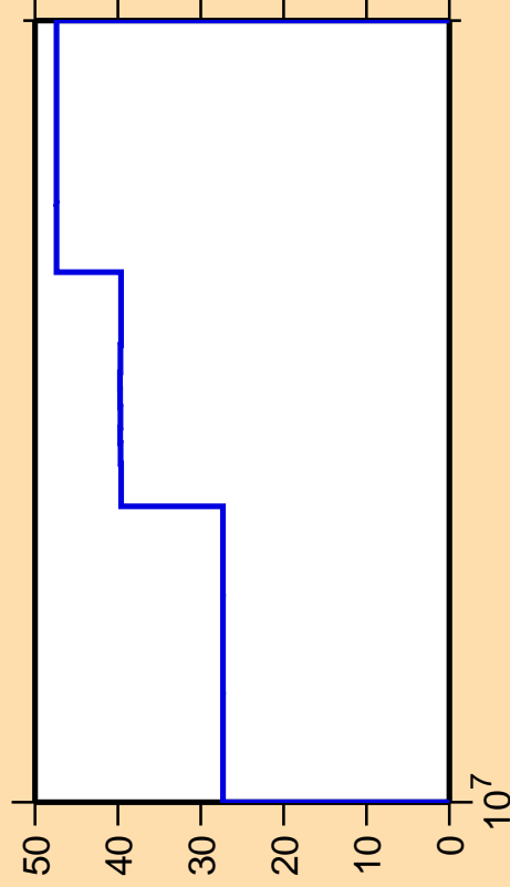
\Delta\sigma/\sigma vs. E for ^{183}\text{Au}(n,n_{\text{cont}})
