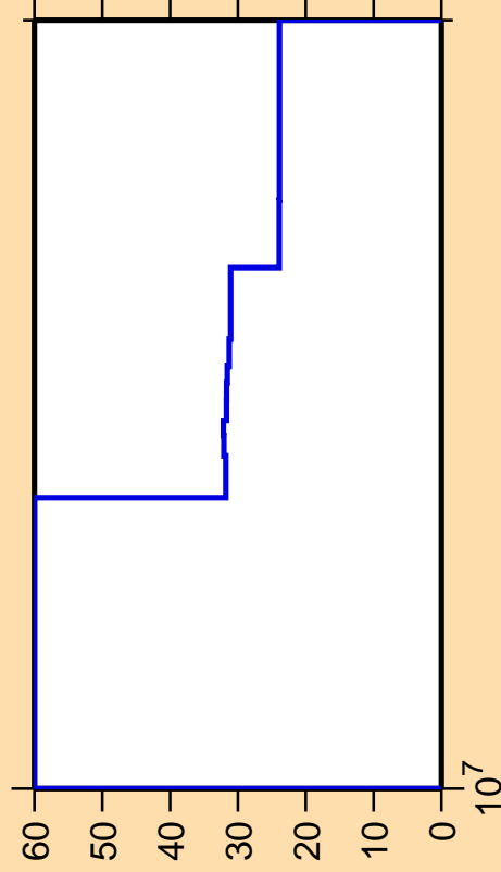
\Delta\sigma/\sigma vs. E for ^{183}\text{Au}(n,2n)
