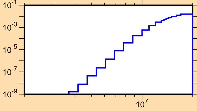
\sigma vs. E for ^{183}\text{Au}(n,d)
