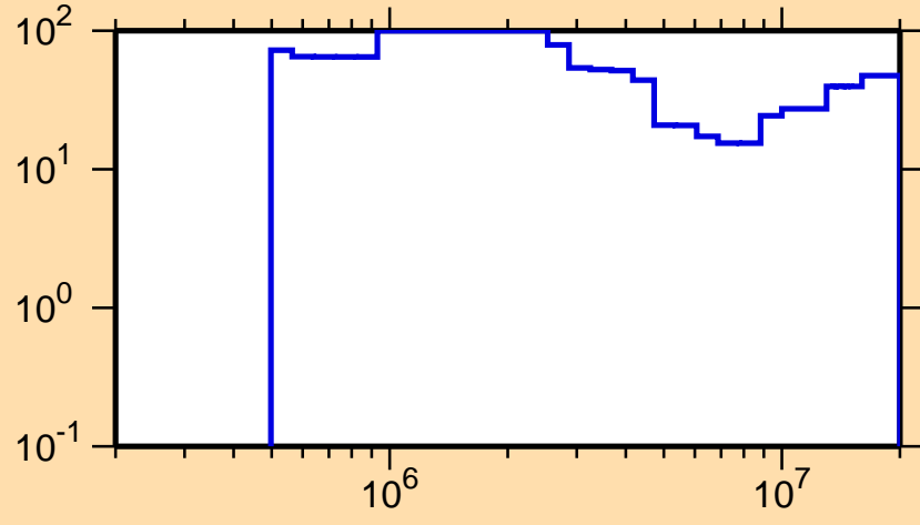
\Delta\sigma/\sigma vs. E for ^{183}\text{Au}(n,n\text{cont.})
