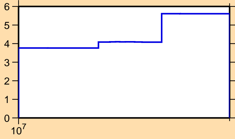
\Delta\sigma/\sigma vs. E for ^{183}\text{Au}(n,\text{tot.})
