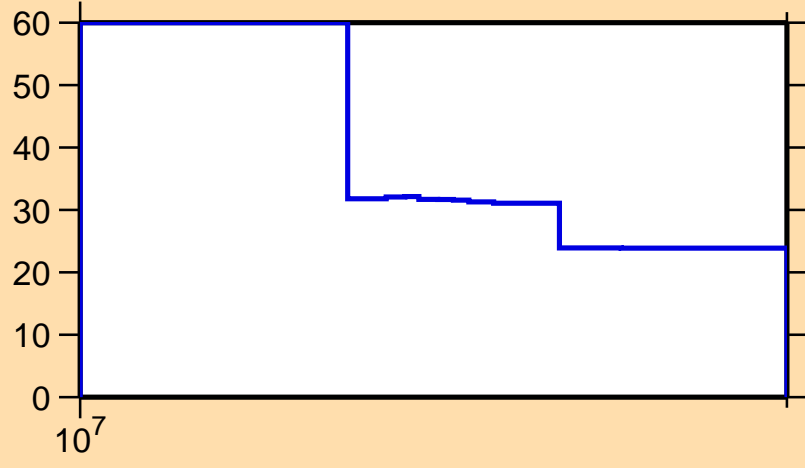
\Delta\sigma/\sigma vs. E for ^{183}\text{Au}(n,2n)
