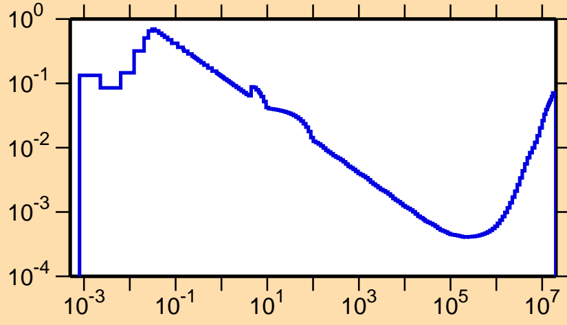
\sigma vs. E for ^{183}\text{Au}(n,\alpha)
