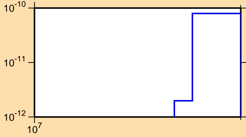
\sigma vs. E for ^{183}\text{Au}(\text{mt } 34)
