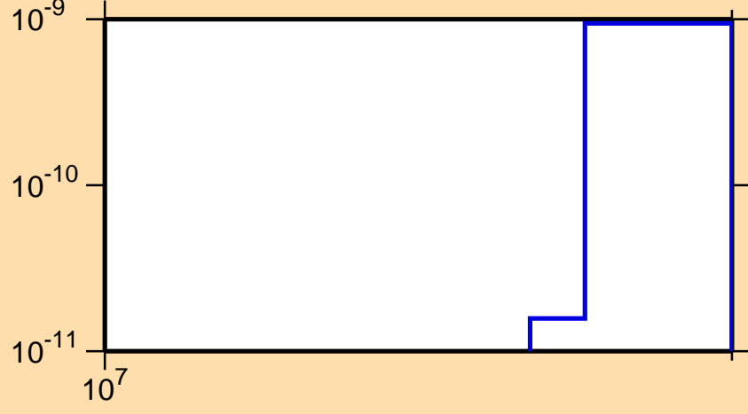
\sigma vs. E for ^{183}\text{Au}(n,pt)
