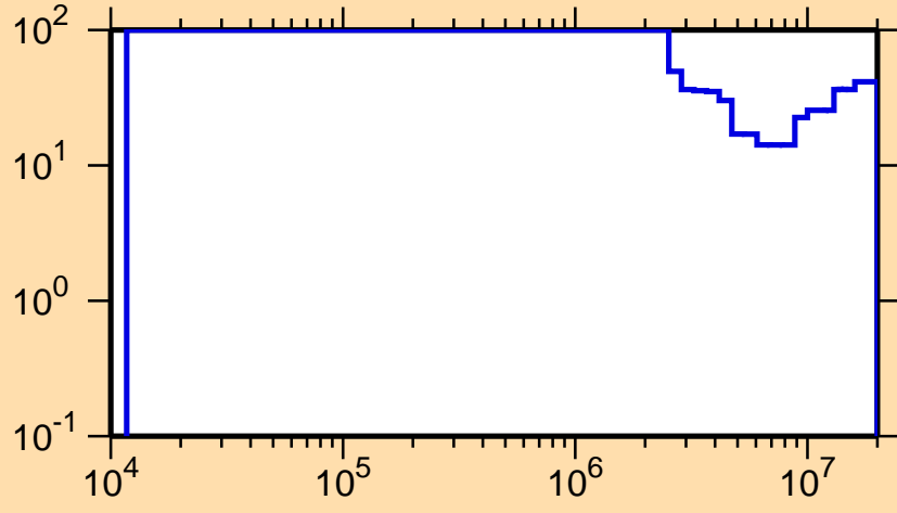
\Delta\sigma/\sigma vs. E for ^{183}\text{Au}(n,\text{inel.})
