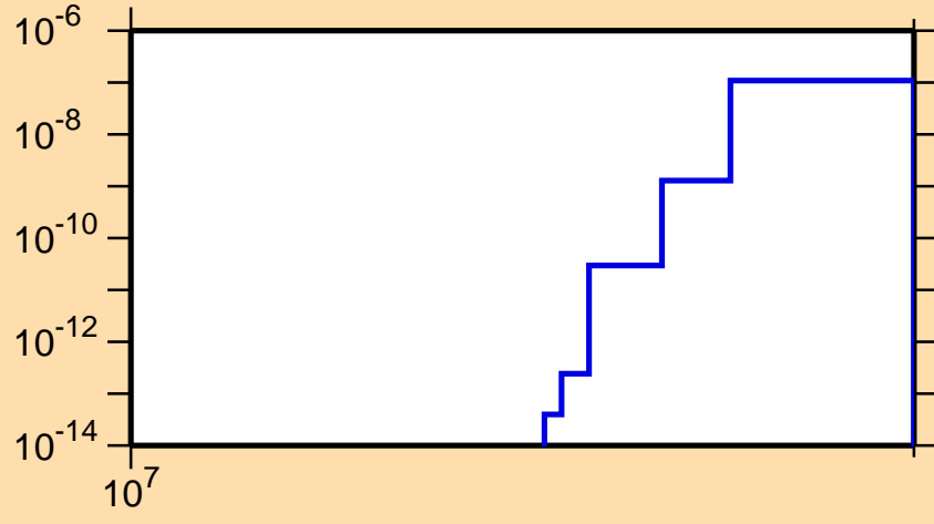
\sigma vs. E for ^{183}\text{Au}(n,nt)
