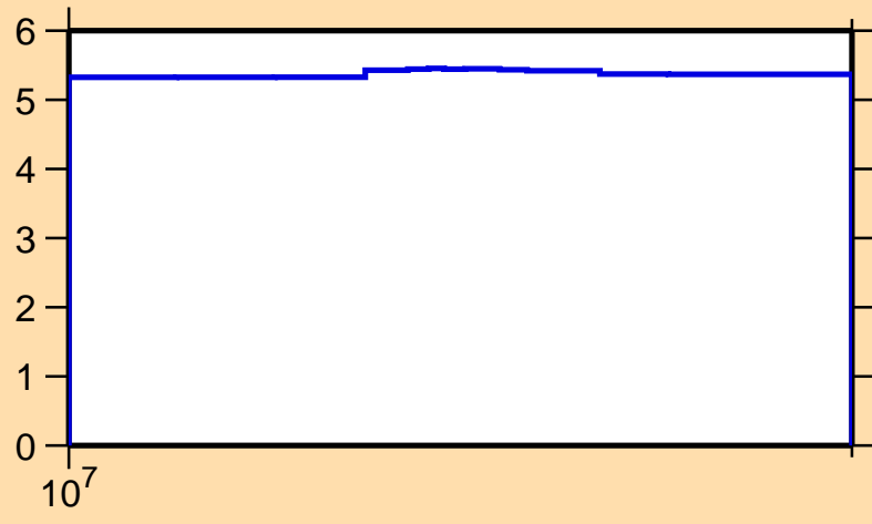
\Delta\sigma/\sigma vs. E for ^{183}\text{Au}(n,\text{nonel.})
