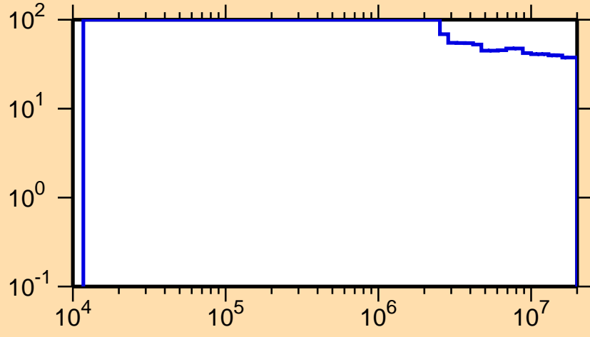
\Delta\sigma/\sigma vs. E for ^{183}\text{Au}(n,n_1)
