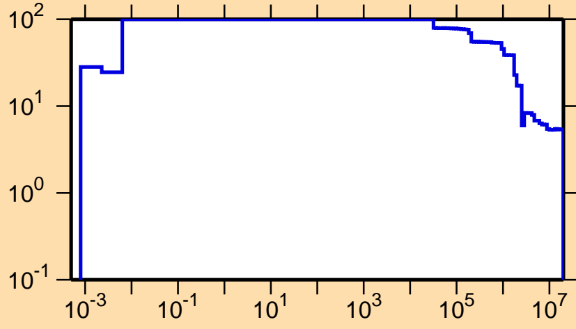
\Delta\sigma/\sigma vs. E for ^{183}\text{Au}(n,\text{nonel.})
