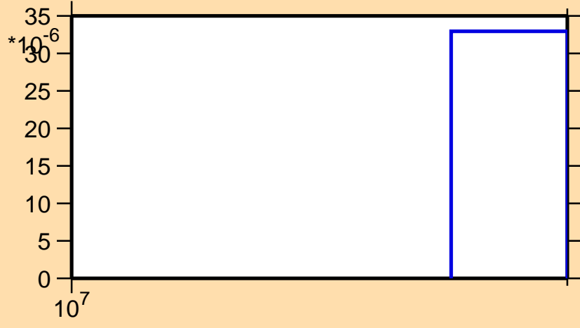
\sigma vs. E for ^{183}\text{Au}(n,3n)
