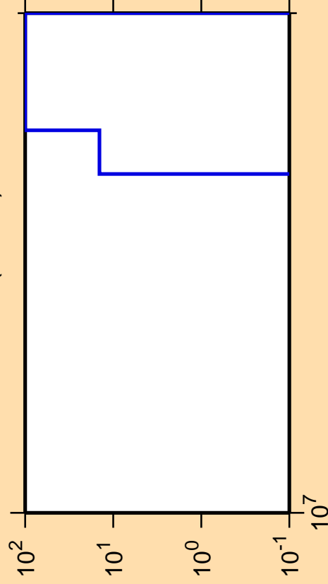
\Delta\sigma/\sigma vs. E for ^{183}\text{Au}(\text{mt } 34)
