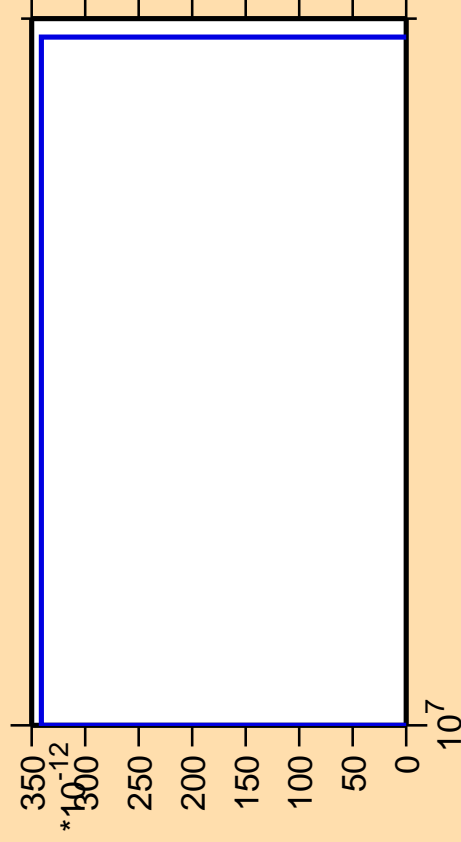
\Delta\sigma/\sigma vs. E for ^{183}\text{Au} (mt 42)
