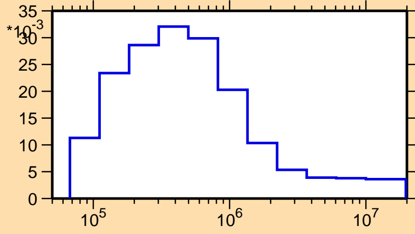
\sigma vs. E for ^{183}\text{Au}(n,n_3)
