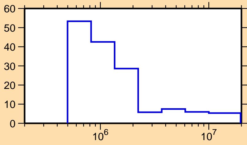
\Delta\sigma/\sigma vs. E for ^{183}\text{Au}(n,\text{nonel.})
