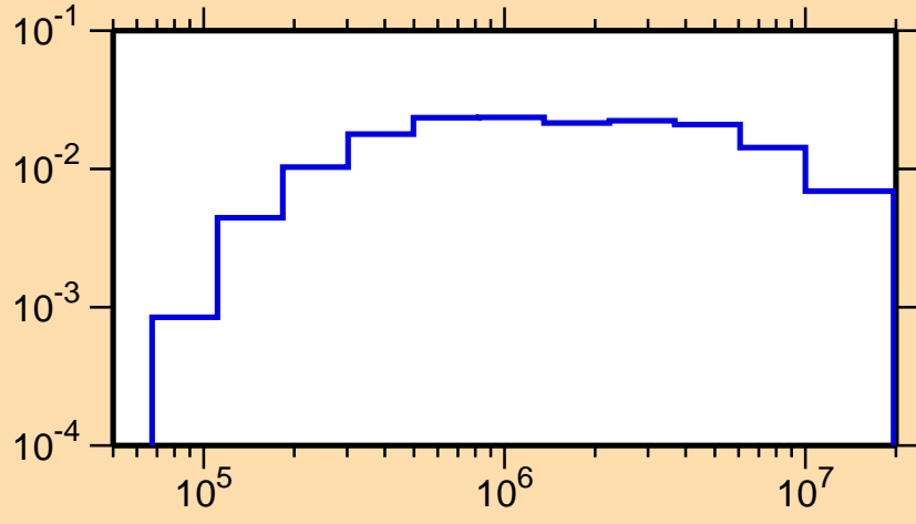
\sigma vs. E for ^{183}\text{Au}(n,n_4)
