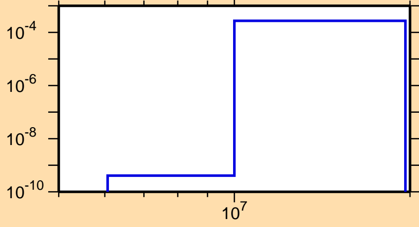
\sigma vs. E for ^{183}\text{Au}(n,t)
