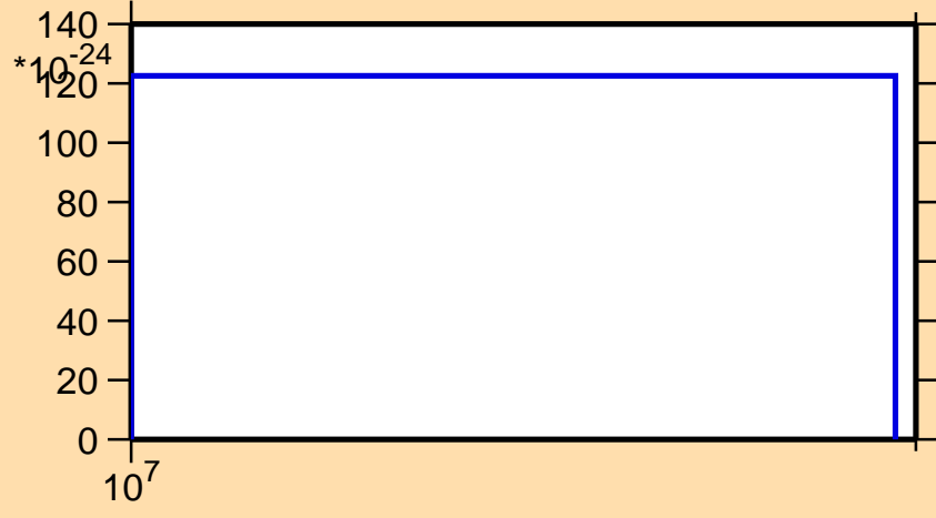
\sigma vs. E for ^{183}\text{Au} (mt 42)
