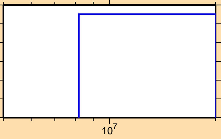
\sigma vs. E for ^{183}\text{Au}(\text{mt117})
