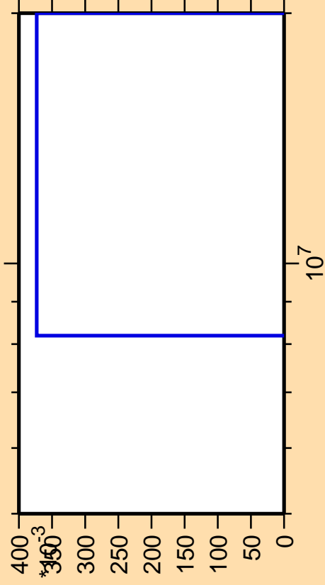
\Delta\sigma/\sigma vs. E for ^{183}\text{Au}(n,3n\alpha)
