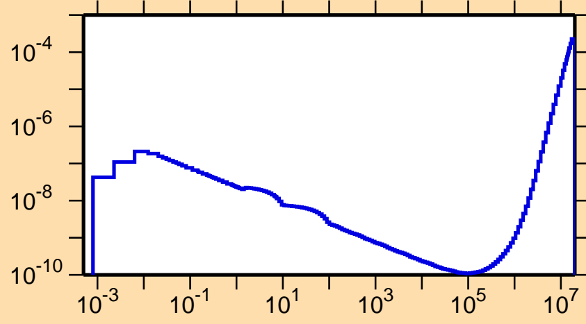
\sigma vs. E for ^{184}\text{Au}(n,p\alpha)
