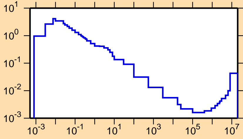
\sigma vs. E for ^{184}\text{Au}(n,\alpha)
