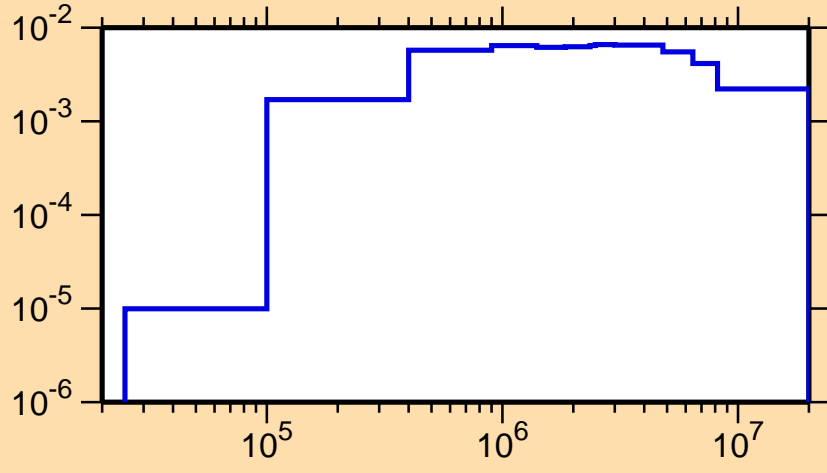
\sigma vs. E for ^{184}\text{Au}(n,n_1)
