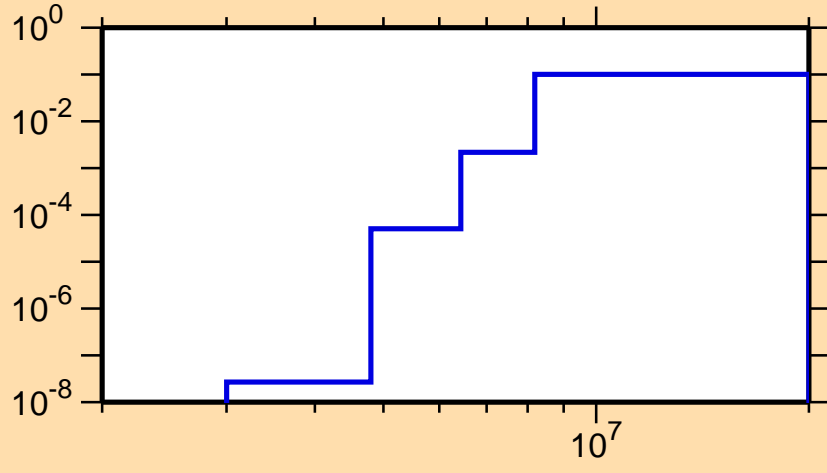
\sigma vs. E for ^{184}\text{Au}(n,np)
