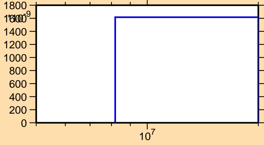
\sigma vs. E for ^{184}\text{Au}(n,nd)
