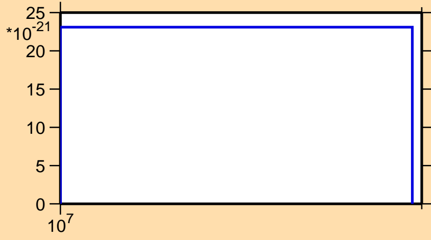
\sigma vs. E for ^{184}\text{Au} (mt 42)
