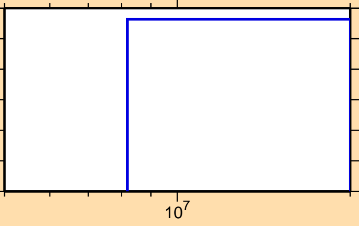
\sigma vs. E for ^{184}\text{Au}(n,\text{pd})
