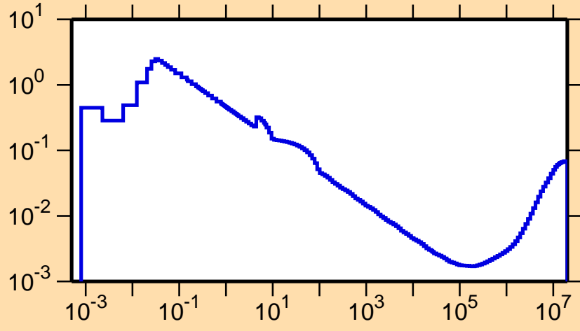
\sigma vs. E for ^{185}\text{Au}(n,p)
