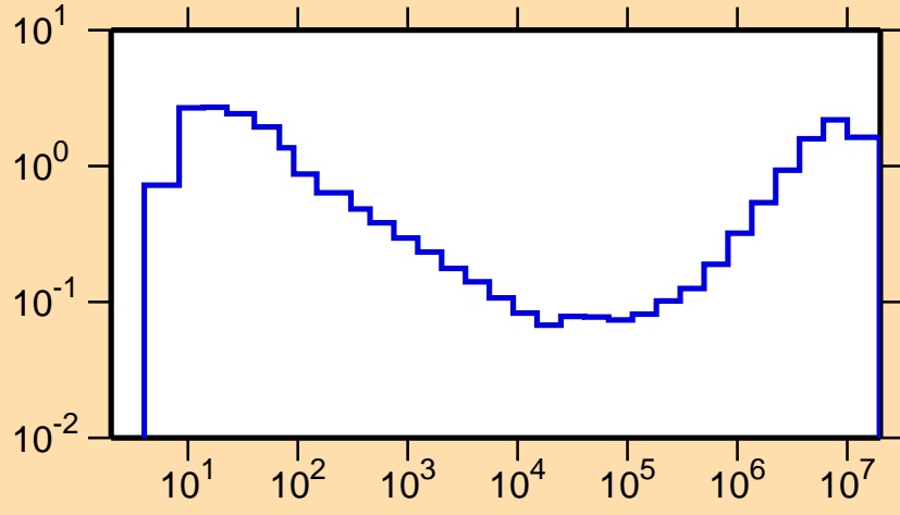
\sigma vs. E for ^{185}\text{Au}(n,\text{inel.})
