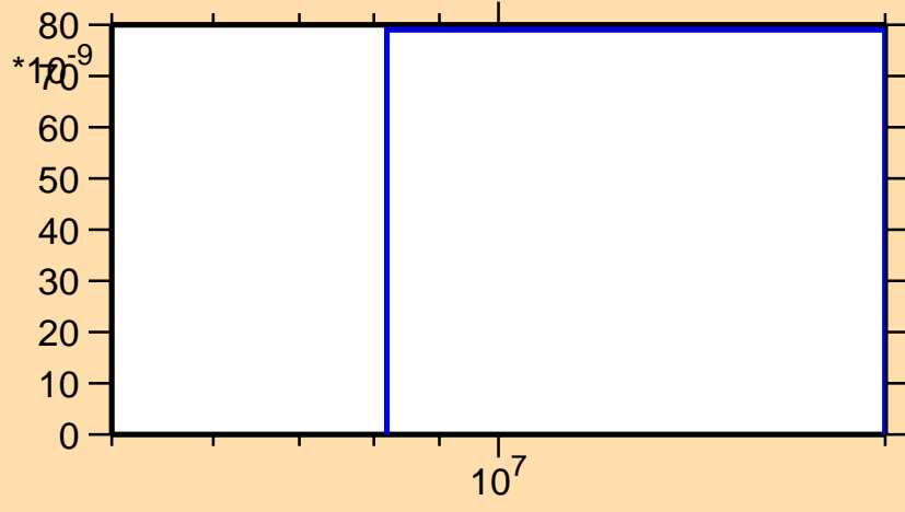
\sigma vs. E for ^{185}\text{Au}(n,nd)
