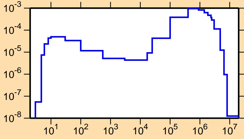
\sigma vs. E for ^{185}\text{Au}(n,n_4)
