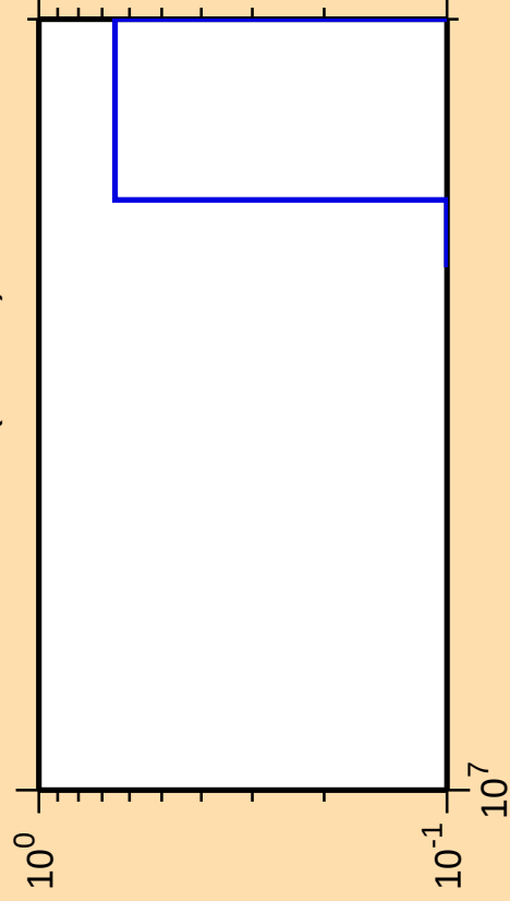
\Delta\sigma/\sigma vs. E for ^{186}\text{Au}(n,3n\alpha)
