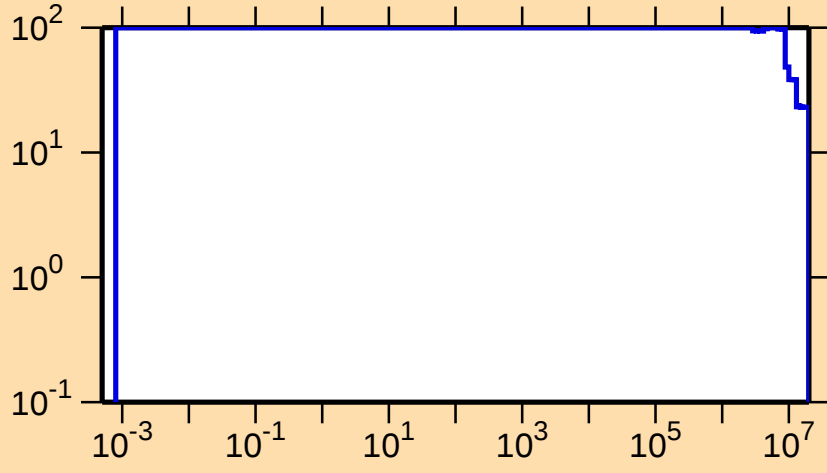
\Delta\sigma/\sigma vs. E for ^{186}\text{Au}(n,p)
