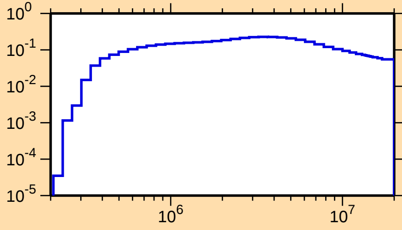
\sigma vs. E for ^{186}\text{Au}(n,n_4)
