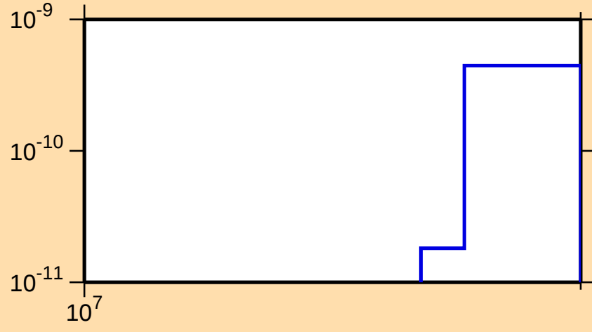
\sigma vs. E for ^{186}\text{Au}(\text{mt } 34)
