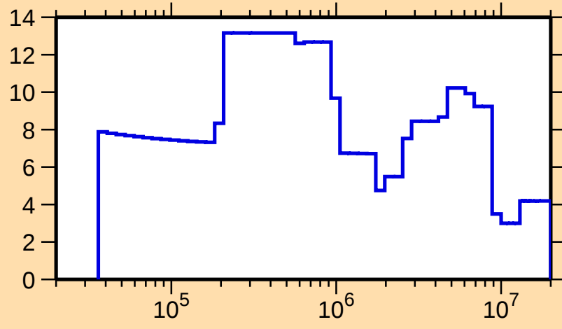
\Delta\sigma/\sigma vs. E for ^{186}\text{Au}(n,\text{tot.})
