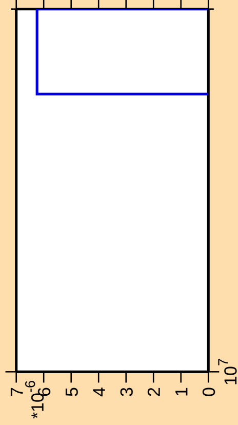
\Delta\sigma/\sigma vs. E for ^{186}\text{Au}(\text{mt } 42)
