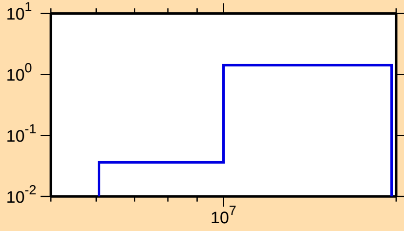
\sigma vs. E for ^{186}\text{Au}(n,2n)
