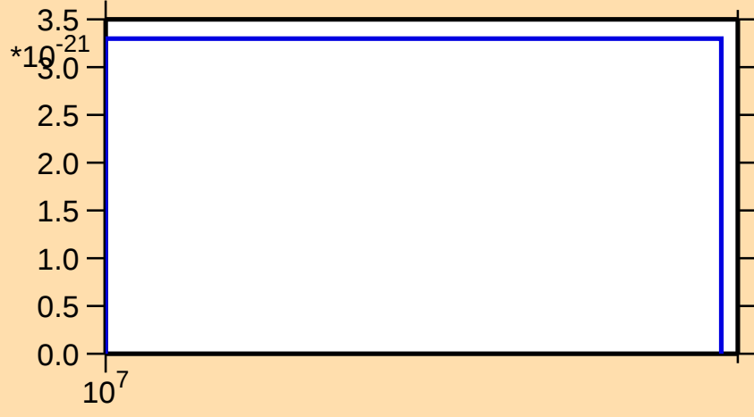
\sigma vs. E for ^{186}\text{Au}(\text{mt } 42)
