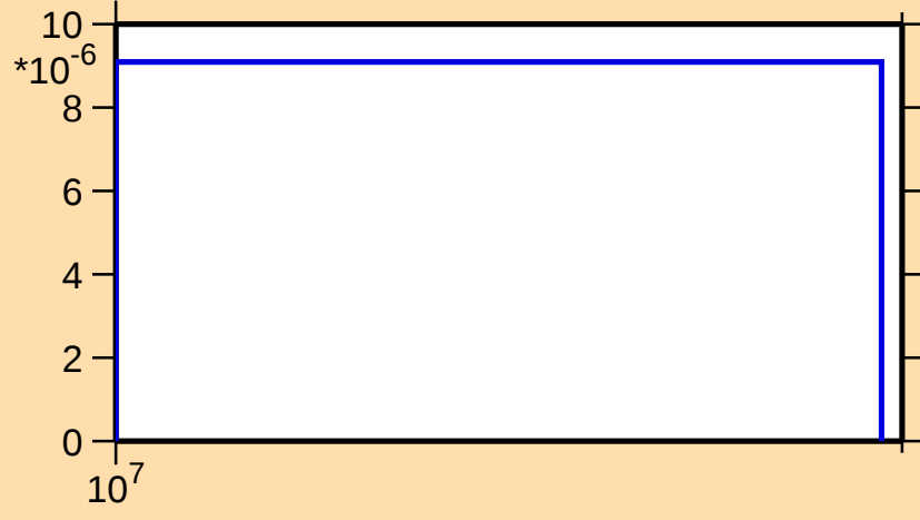
\sigma vs. E for ^{186}\text{Au}(n,3n)
