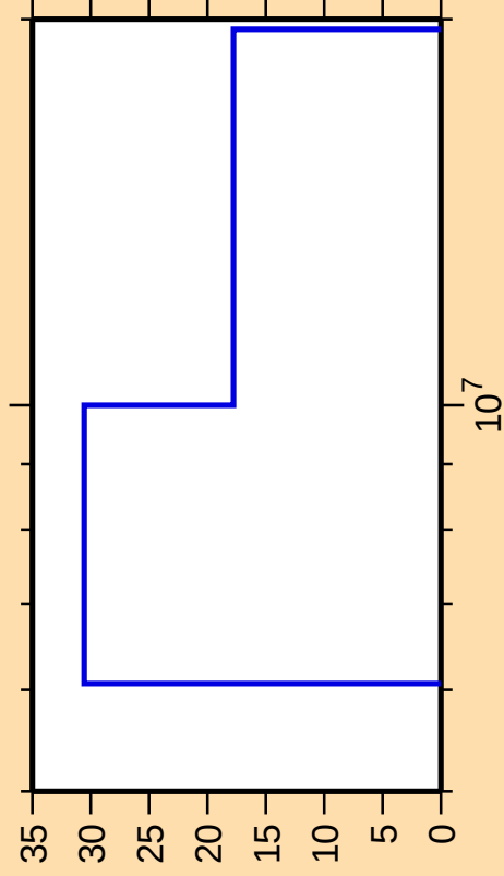
\Delta\sigma/\sigma vs. E for ^{186}\text{Au}(n,2n)
