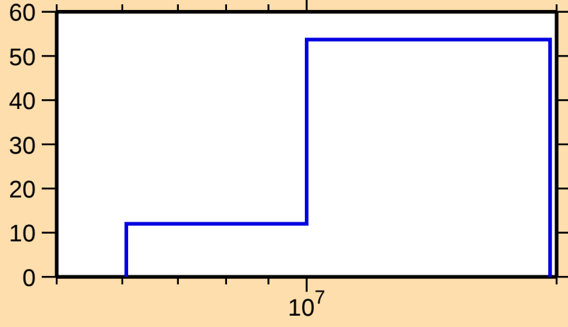
\Delta\sigma/\sigma vs. E for ^{186}\text{Au}(n,\text{inel.})
