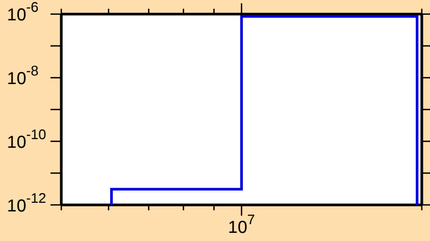
\sigma vs. E for ^{186}\text{Au}(n,\text{He3})
