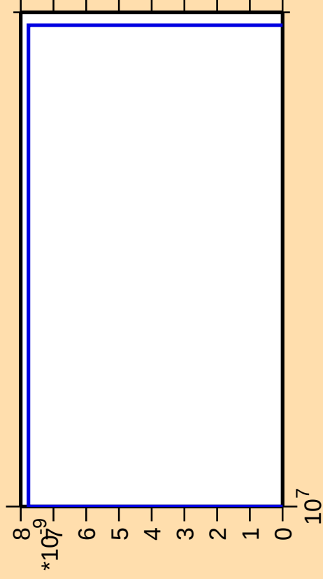
\Delta\sigma/\sigma vs. E for ^{186}\text{Au}(\text{mt } 42)
