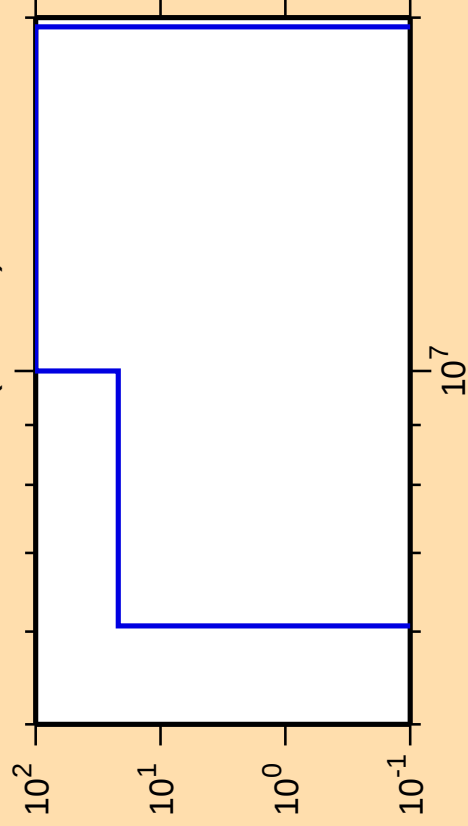
\Delta\sigma/\sigma vs. E for ^{186}\text{Au}(n,\text{He3})
