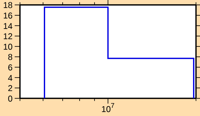
\Delta\sigma/\sigma vs. E for ^{186}\text{Au}(n,\text{el.})
