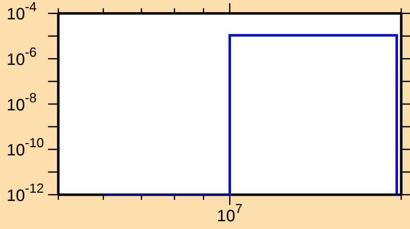
\sigma vs. E for ^{186}\text{Au}(n,2n\alpha)
