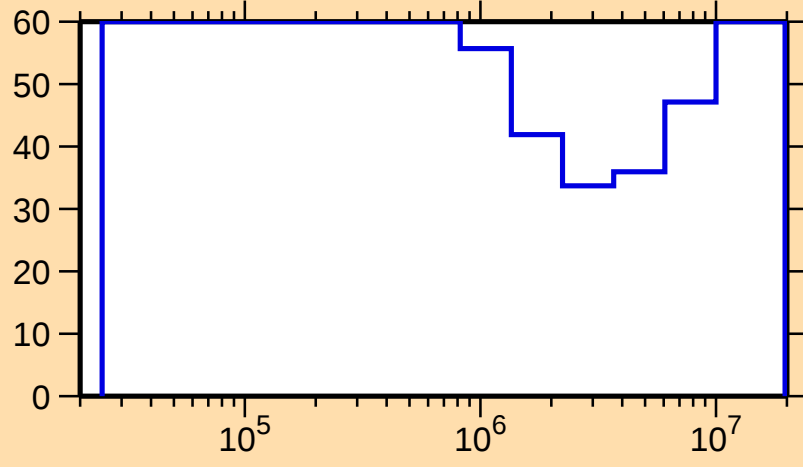
\Delta\sigma/\sigma vs. E for ^{186}\text{Au}(n,n_1)
