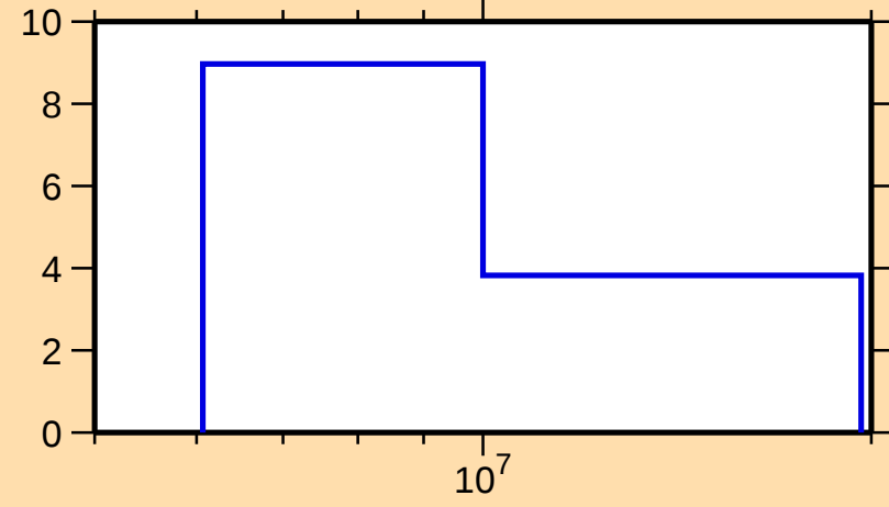
\Delta\sigma/\sigma vs. E for ^{186}\text{Au}(n,\text{tot.})
