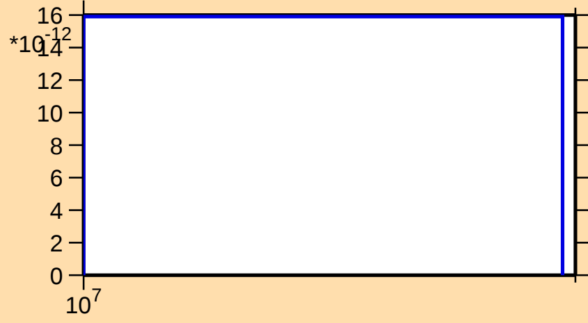
\sigma vs. E for ^{186}\text{Au}(n,\text{pt})
