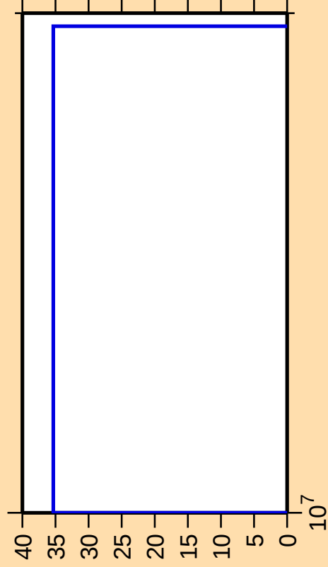
\Delta\sigma/\sigma vs. E for ^{186}\text{Au}(\text{mt } 34)
