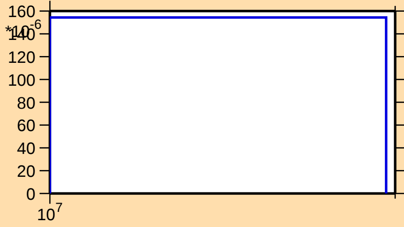
\sigma vs. E for ^{186}\text{Au}(n,2np)
