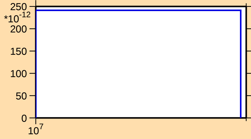
\sigma vs. E for ^{186}\text{Au}(n,\text{pd})
