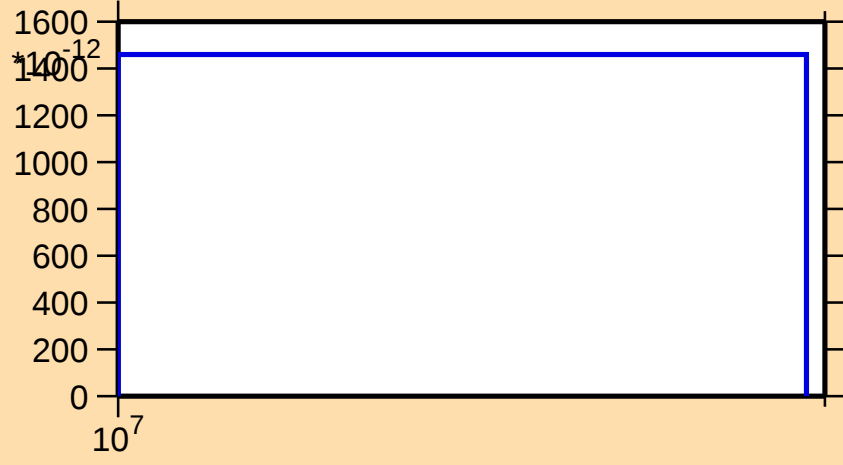
\sigma vs. E for ^{186}\text{Au}(n,nt)
