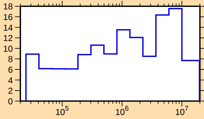
\Delta\sigma/\sigma vs. E for ^{186}\text{Au}(n,\text{el.})
