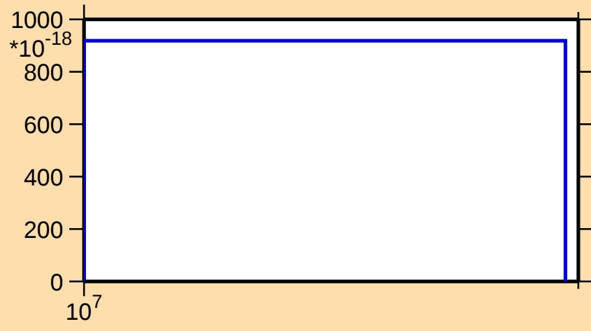
\sigma vs. E for ^{186}\text{Au}(n,3n\alpha)
