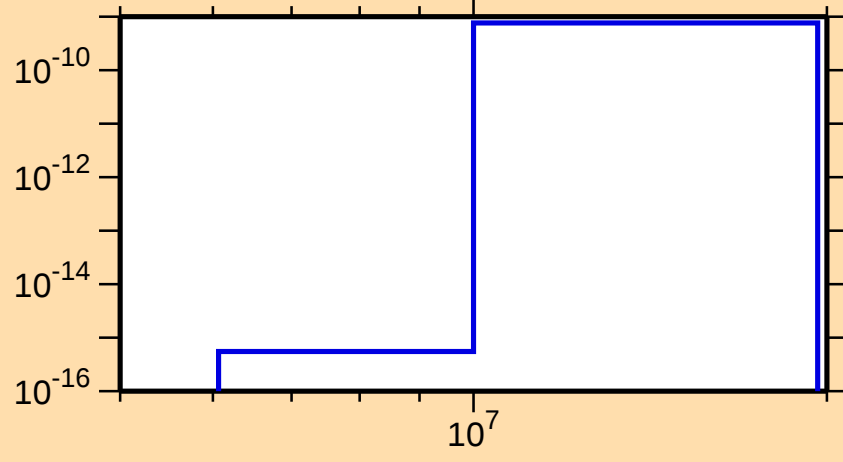
\sigma vs. E for ^{186}\text{Au}(\text{mt117})
