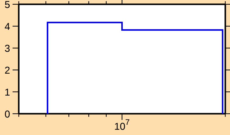
\Delta\sigma/\sigma vs. E for ^{186}\text{Au}(n,\text{nonel.})
