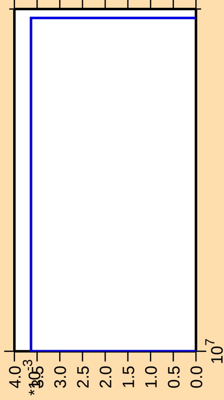
\Delta\sigma/\sigma vs. E for ^{186}\text{Au}(n,3n\alpha)
