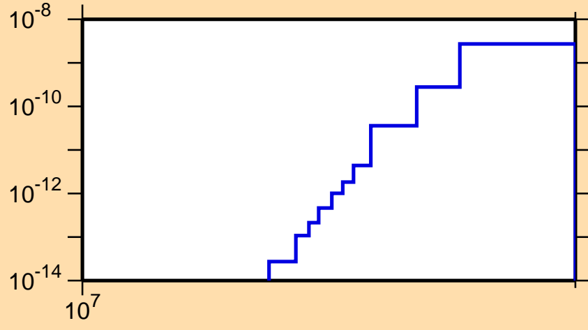
\sigma vs. E for ^{187}\text{Au}(n,\text{pd})
