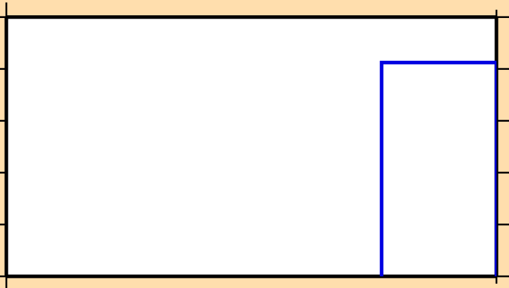
\sigma vs. E for ^{187}\text{Au}(n,3n)
