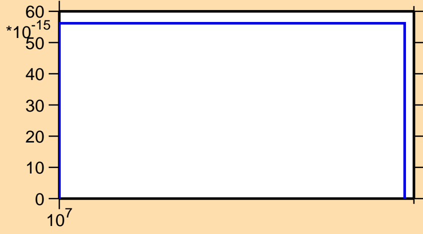
\sigma vs. E for ^{187}\text{Au}(n,pt)
