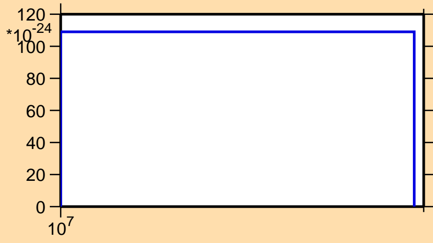
\sigma vs. E for ^{187}\text{Au} (mt 42)
