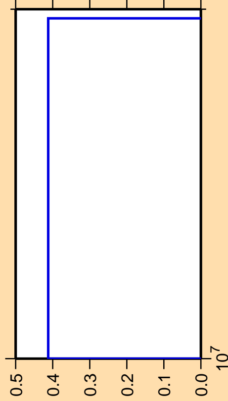
\Delta\sigma/\sigma vs. E for ^{187}\text{Au}(n,pt)
