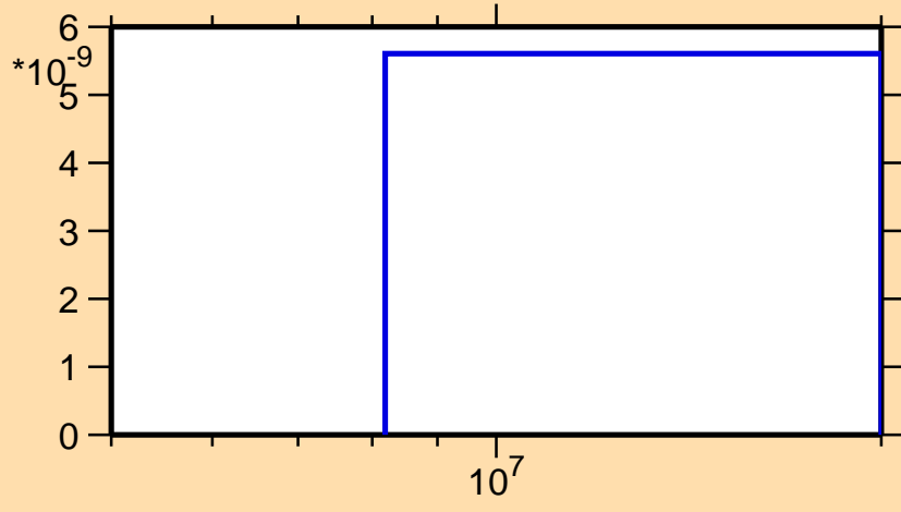
\sigma vs. E for ^{187}\text{Au}(\text{mt } 45)
