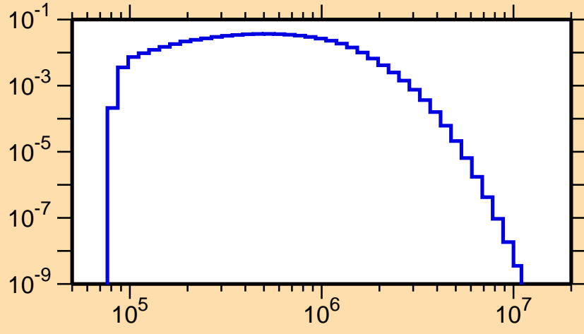
\sigma vs. E for ^{188}\text{Au}(n,n_2)
