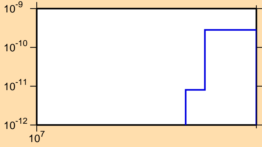
\sigma vs. E for ^{188}\text{Au}(n,\text{pt})
