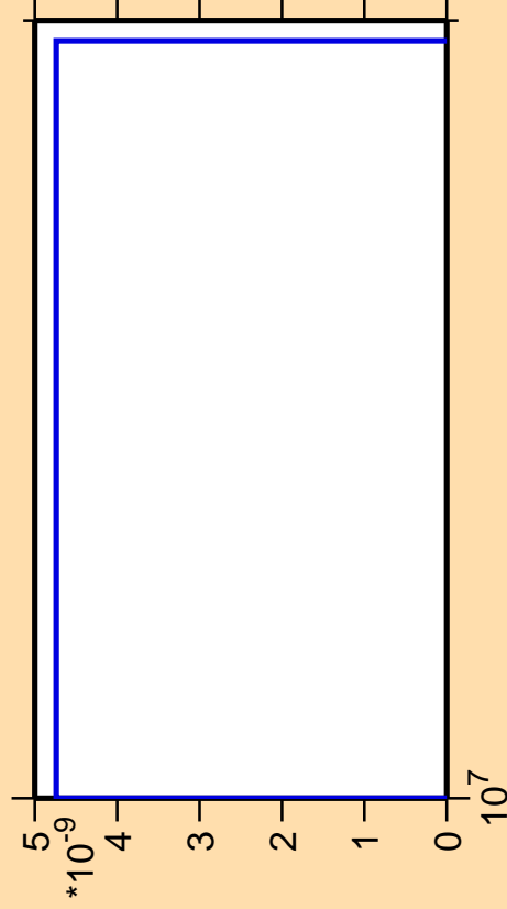
\Delta\sigma/\sigma vs. E for ^{188}\text{Au} (mt 42)
