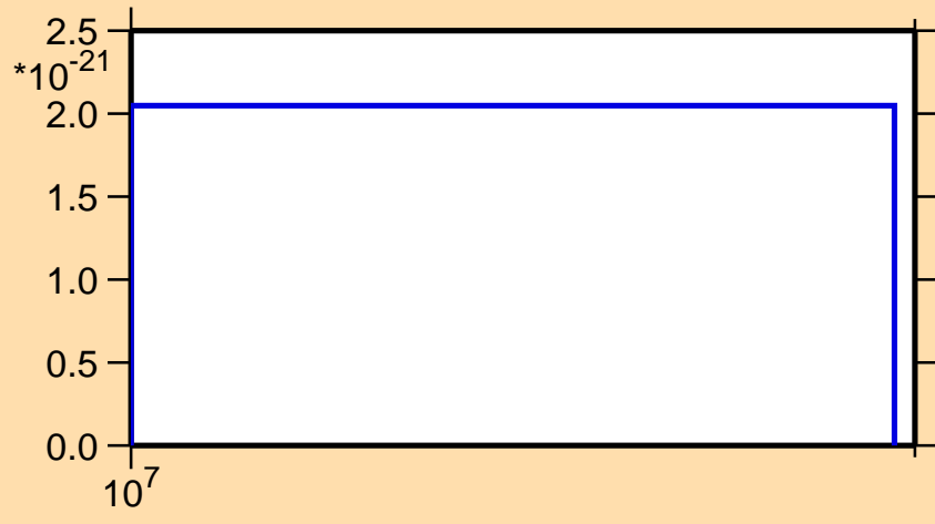
\sigma vs. E for ^{188}\text{Au} (mt 42)
