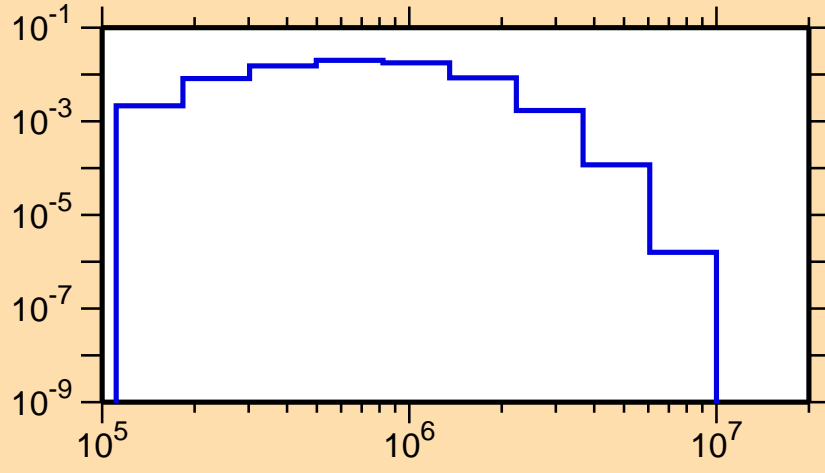
\sigma vs. E for ^{188}\text{Au}(n,n_3)
