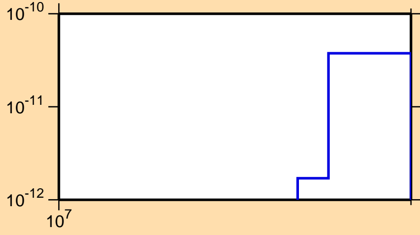
\sigma vs. E for ^{189}\text{Au}(n,\text{pd})
