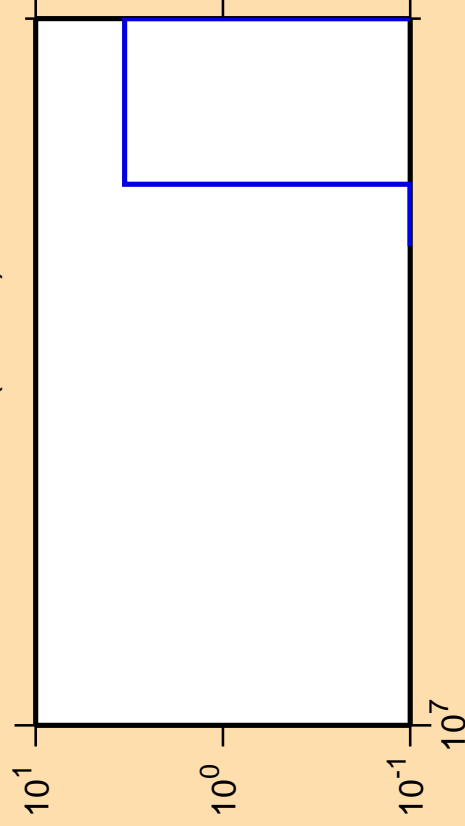
\Delta\sigma/\sigma vs. E for ^{189}\text{Au}(\text{mt } 34)
