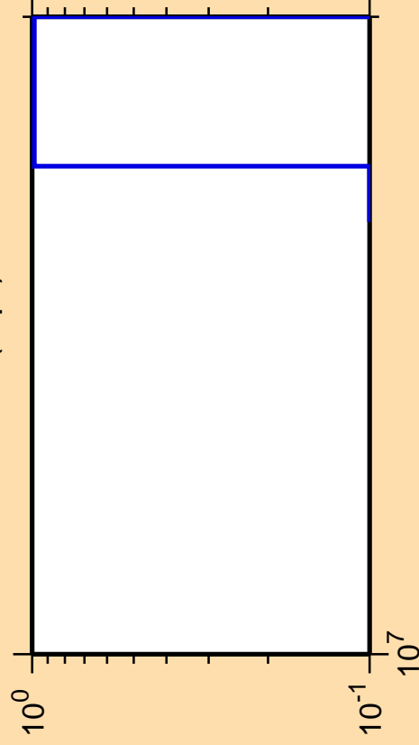
\Delta\sigma/\sigma vs. E for ^{189}\text{Au}(n,\text{pt})
