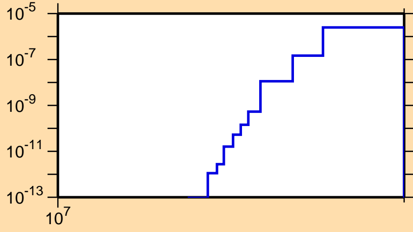
\sigma vs. E for ^{189}\text{Au}(n,\text{nd})
