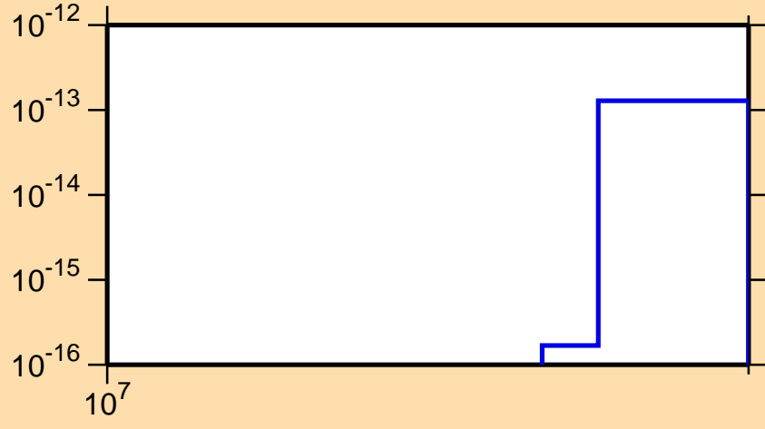
\sigma vs. E for ^{189}\text{Au}(n,\text{pt})
