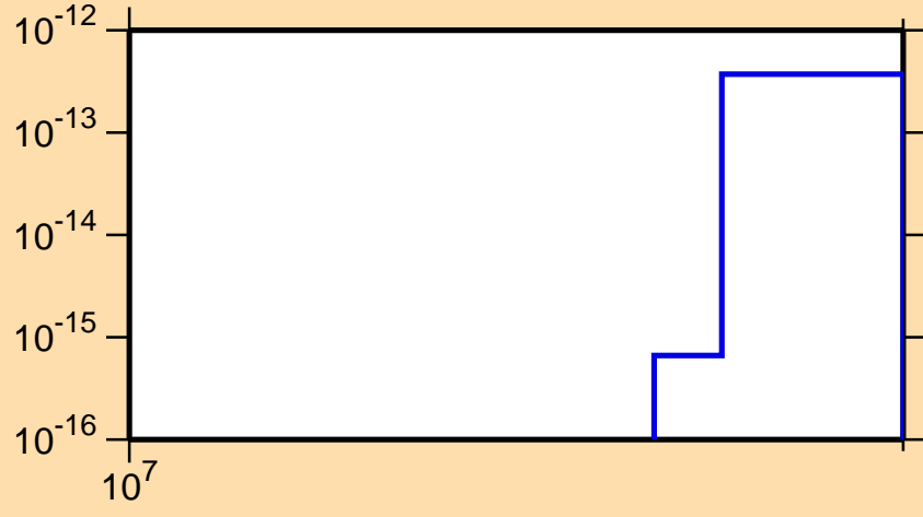
\sigma vs. E for ^{189}\text{Au}(\text{mt } 34)
