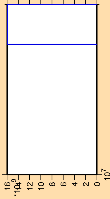
\Delta\sigma/\sigma vs. E for ^{189}\text{Au} (mt 42)
