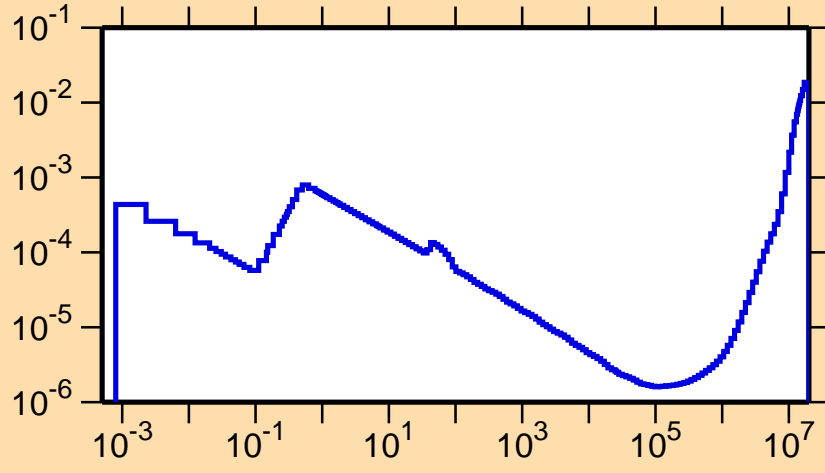
\sigma vs. E for ^{189}\text{Au}(n,\alpha)
