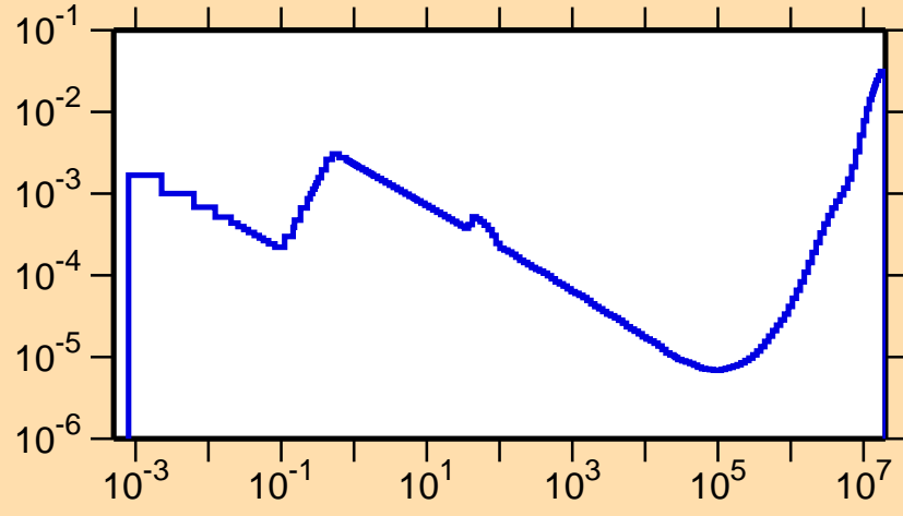
\sigma vs. E for ^{189}\text{Au}(n,p)
