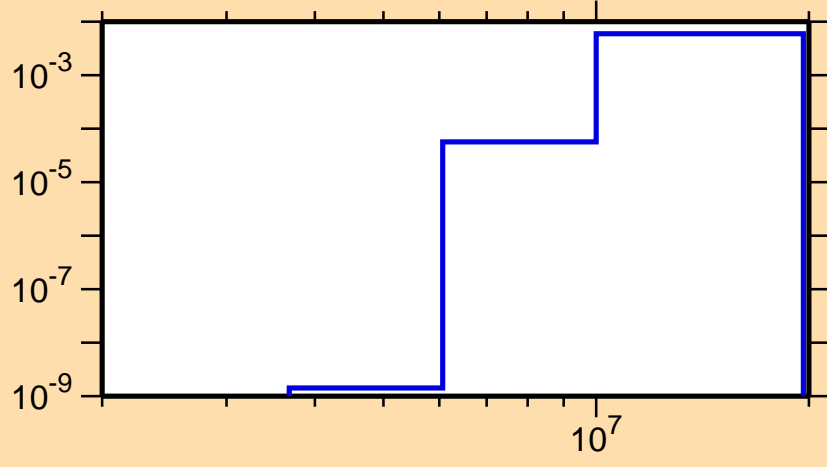
\sigma vs. E for ^{189}\text{Au}(n,np)
