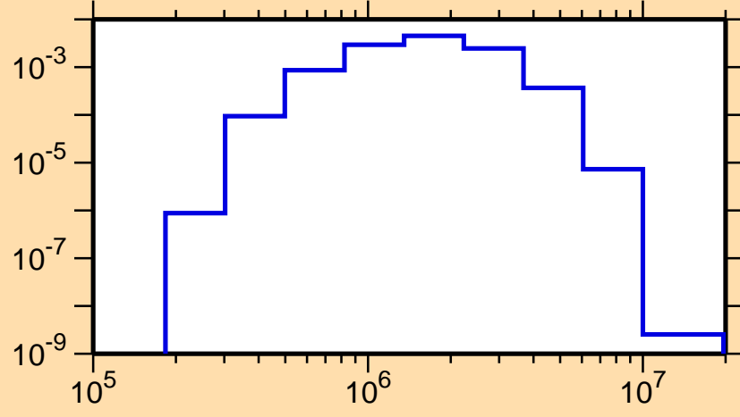
\sigma vs. E for ^{189}\text{Au}(n,n_3)
