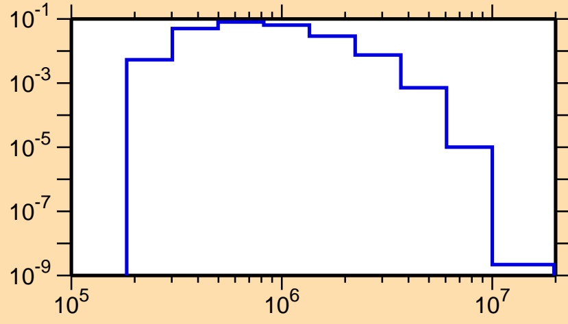
\sigma vs. E for ^{189}\text{Au}(n,n_4)
