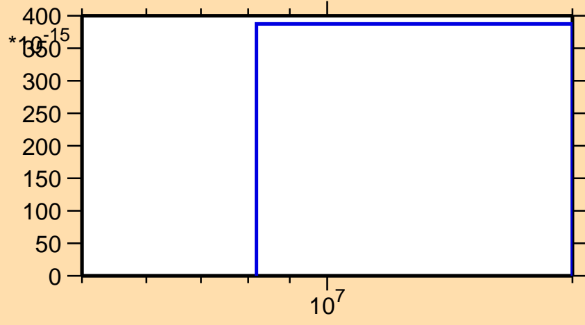
\sigma vs. E for ^{189}\text{Au}(n,pd)
