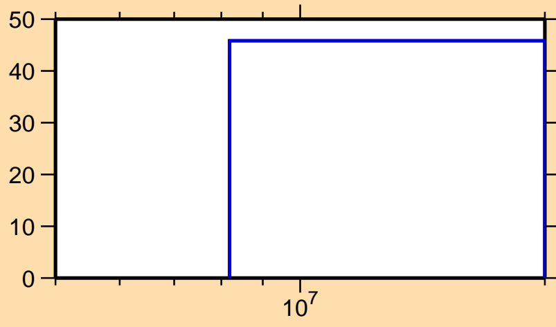
\Delta\sigma/\sigma vs. E for ^{189}\text{Au}(n,2n)
