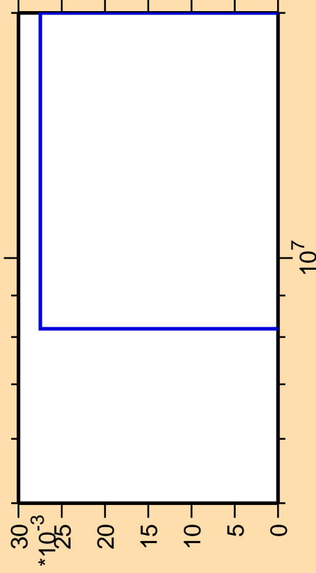
\Delta\sigma/\sigma vs. E for ^{189}\text{Au}(\text{mt } 34)
