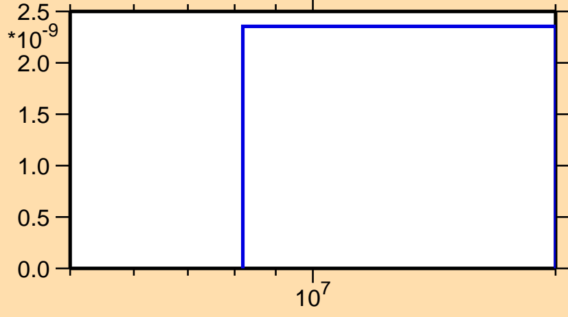
\sigma vs. E for ^{189}\text{Au}(n,nt)
