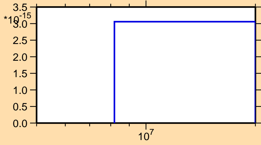
\sigma vs. E for ^{189}\text{Au}(\text{mt } 34)
