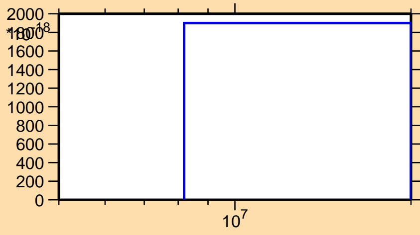
\sigma vs. E for ^{189}\text{Au}(n,3n\alpha)
