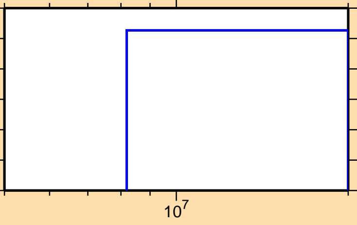
\sigma vs. E for ^{189}\text{Au}(n,\text{pt})
