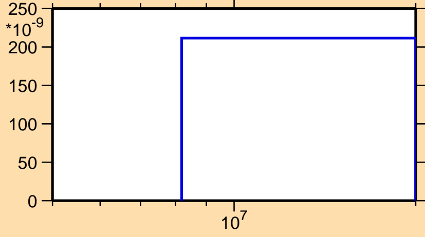
\sigma vs. E for ^{189}\text{Au}(n,2n\alpha)
