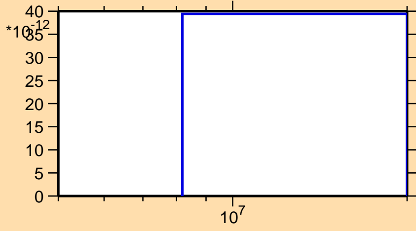
\sigma vs. E for ^{189}\text{Au}(\text{mt117})
