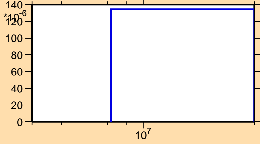
\sigma vs. E for ^{189}\text{Au}(n,3n)
