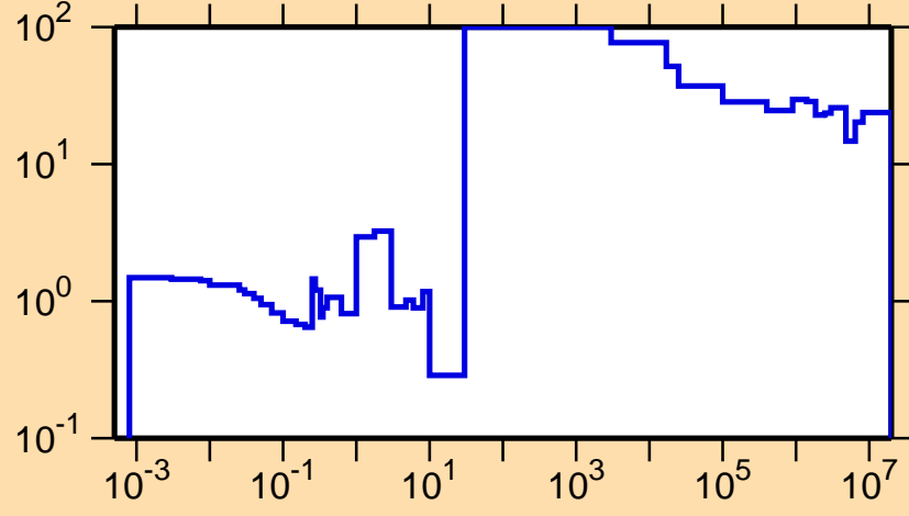
\Delta\sigma/\sigma vs. E for ^{189}\text{Au}(n,\text{el.})
