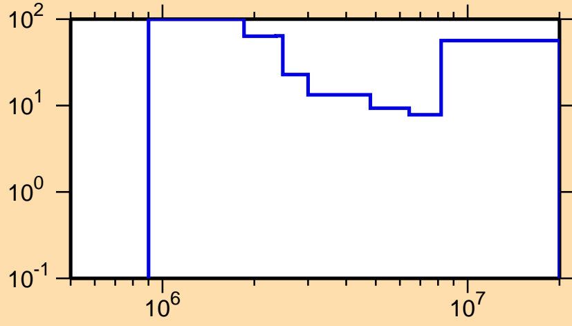
\Delta\sigma/\sigma vs. E for ^{189}\text{Au}(n,n\text{cont.})
