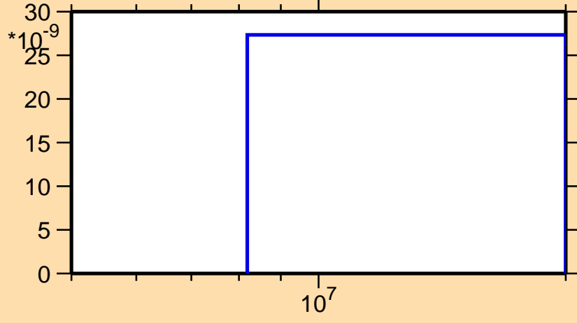
\sigma vs. E for ^{189}\text{Au}(n,nd)
