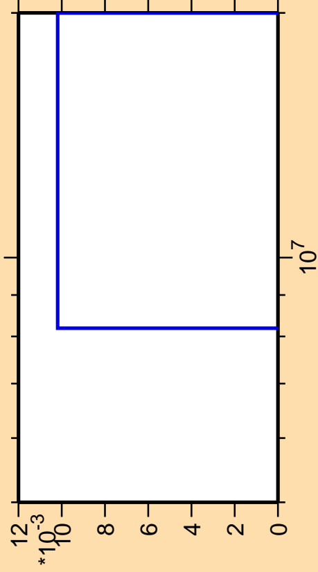
\Delta\sigma/\sigma vs. E for ^{189}\text{Au}(n,3n\alpha)
