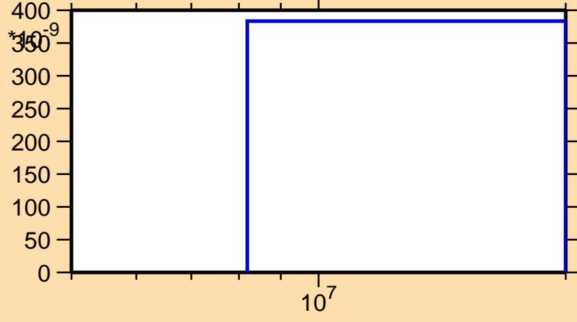
\sigma vs. E for ^{189}\text{Au}(n,2np)
