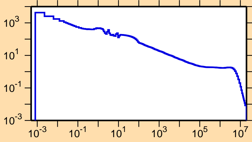
\sigma vs. E for ^{189}\text{Au}(n,\gamma)
